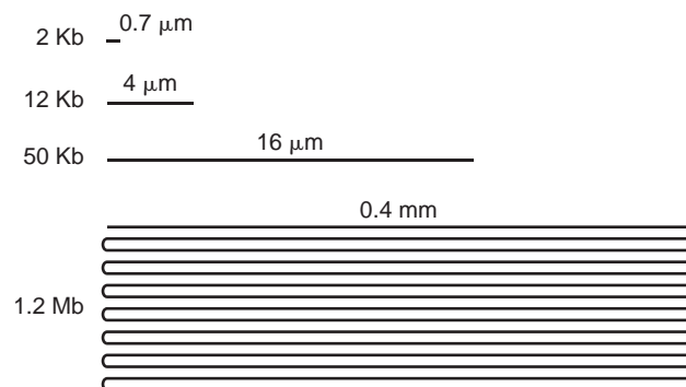
Figure 3.2 Size variation of viral genomes. Lines are drawn in proportion to genome lengths. Genome sizes in kb (thousands of nucleotides) are shown on left, and genome lengths in micrometers ( \mu\text{m} ) or mm are shown above each line. From top to bottom: circoviruses have genomes of less than 2 kb; many positive-strand RNA viruses have genomes of approximately 12 kb; medium-size bacteriophages such as lambda have genomes of 50 kb; the largest known viral genome, that of mimivirus, is 1.2 Mb long.
