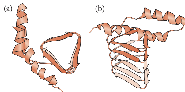
Figure 32.6 \beta -helical model of \text{PrP} 27–30. (a, b) Top and side views, respectively, of \text{PrP} 27–30 modeled with the N-terminal portion of the protein as a left-handed \beta -helix (ribbon arrows displayed in a triangular barrel). The structure of the \alpha -helical part (ribbon helices) was derived from the known structure of the C-terminal region of \text{PrP}^{\text{C}} .
