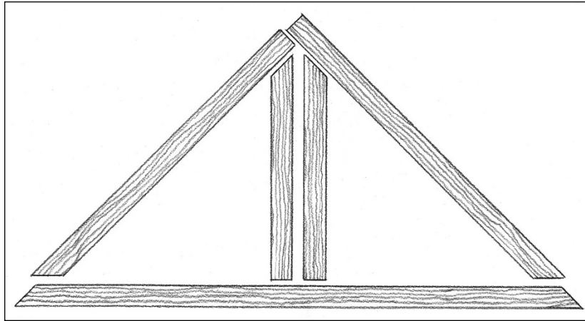
FIGURE 5-2: Sleeping shelf frame assembly.
