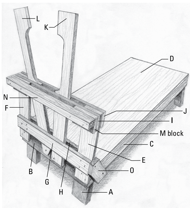
FIGURE 4-2: A milk stand.
