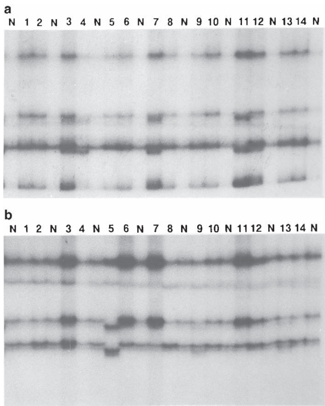
Fig. 6.20 Single-strand conformation polymorphism analysis of polymerase chain reaction-amplified Kirsten- ras exon 1 from intrahepatic bile duct lesions in hamsters. (a) Papillary adenocarcinoma of the intrahepatic bile duct. Lanes 3, 4, 7, 11, 12, shifted bands in addition to normal ones (N). (b) Tubular hyperplasia of the intrahepatic bile duct. Lanes 5, 9, 13, shifted bands in addition to normal ones (N) ([17], with permission)
