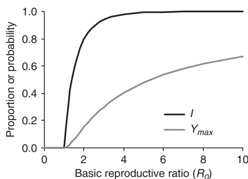
Fig. 3.1. The probability that an animal is infected during an epidemic ( I ) and the maximum proportion of animals infected at any time point ( Y_{max} ) as a function of the basic reproductive ratio.
