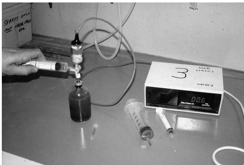
Fig. 11.3. Gas production equipment. (After Theodorou and France, 1993.)
