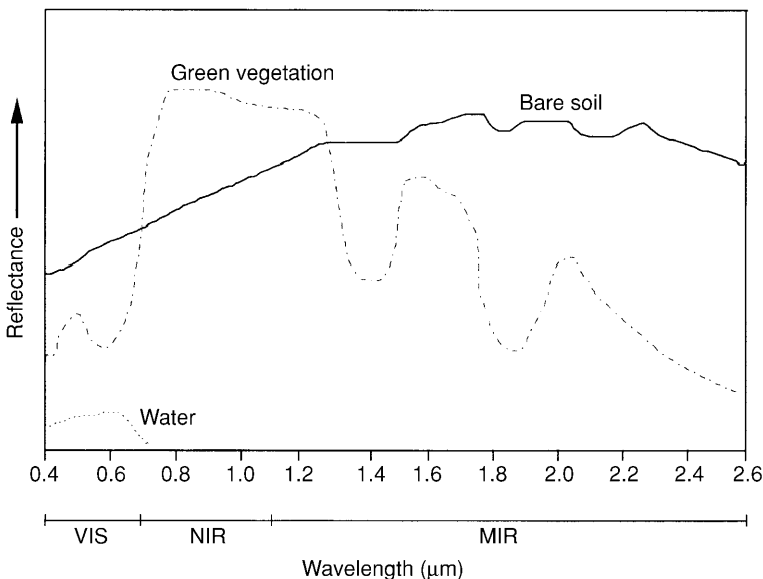
Fig. 9.2. Typical reflectance spectra for green vegetation, soil and water in the VIS–NIR–MIR. (Reproduced from Smith, 1997, with permission of Royal Society of Western Australia.)
