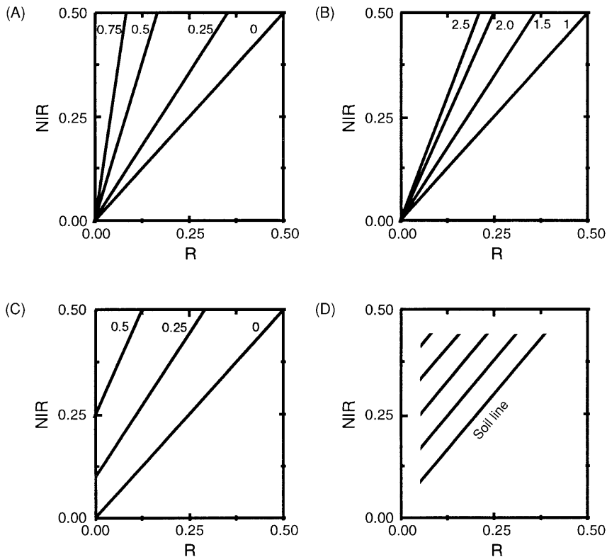
Fig. 9.6. Geometric interpretation of some commonly used vegetation indices (note that, in formulae, N = \text{NIR} ; R = \text{red} ). (A) Normalized difference vegetation index (NDVI) = (N - R) / (N + R) . The NDVI ranges from -1 to 1 and has a nominal soil line at 0. (B) Simple ratio (SR) = N / R . The simple ratio ranges from -\infty to \infty and has a nominal soil line at 1. (C) Soil adjusted vegetation index (SAVI) = (1 + L)(N - R) / (N + R + L) , and L = 0.5 was used. The range and soil line are as for NDVI. (D) The perpendicular vegetation index (PVI) is based on the image analyst identifying the soil line; contours are then computed parallel to this soil line (see Richardson and Weigand, 1977, for details).
