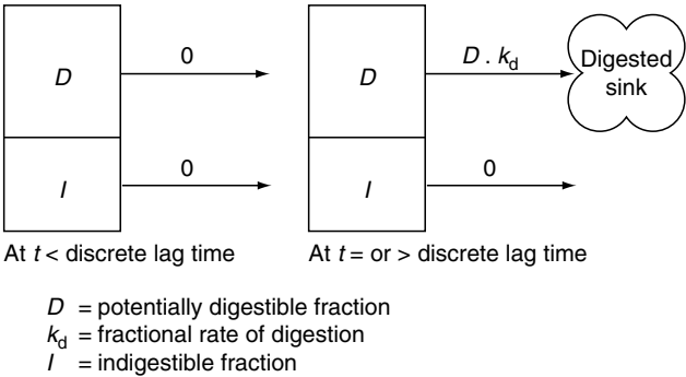
Fig. 2.4. Model 3: Simple first-order model of digestion with a discrete lag time before digestion and an indigestible fraction.
