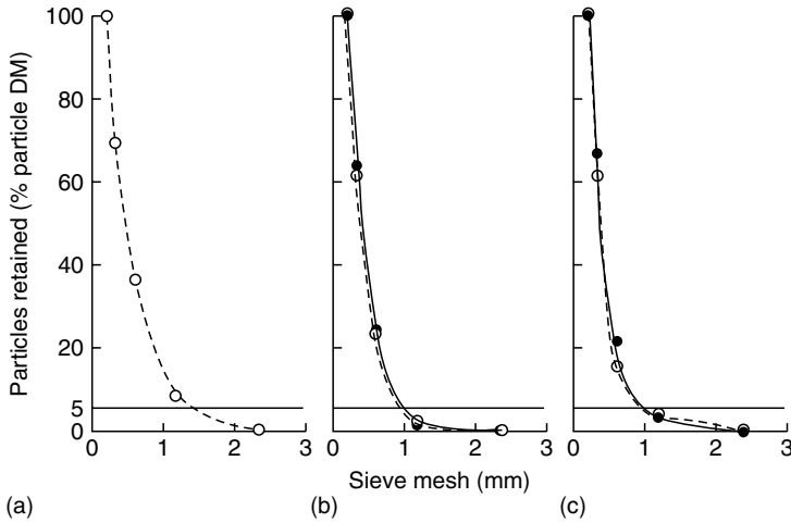
Fig. 3.1. Cumulative particle size distribution in: (a) faeces from grazing cattle; (b) faeces from sheep given chopped (○- - -○) or ground (●- - -●) lucerne hay (Van Soest, 1982); and (c) digesta leaving the stomach of sheep given chopped (○- - -○) or ground and pelleted (●- - -●) lucerne hay.
