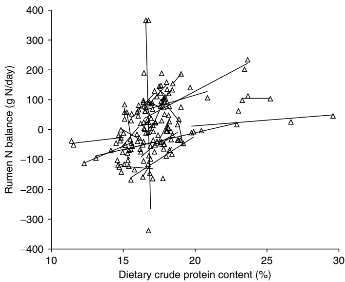
Fig. 10.6. Relationship between crude protein content of the diet (%) and observed rumen N balance (defined as N consumed minus duodenal flow of N, g N per day). Regression of the full data set resulted in the relationship: rumen N balance = 13.83 \times crude protein content - 226.75 ( R^2 = 0.12 ).
