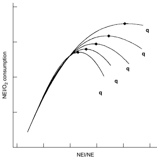
Fig. 23.3. Efficiency of oxygen utilization (net energy intake/ O_2 consumption) as a function of net energy intake (NEI) scaled to net energy for maintenance ( NE_m ), for foods with five metabolizabilities (Tolkamp and Ketelaars, 1992). ◆, Observed voluntary intakes of such feeds (Agricultural Research Council, 1980).
