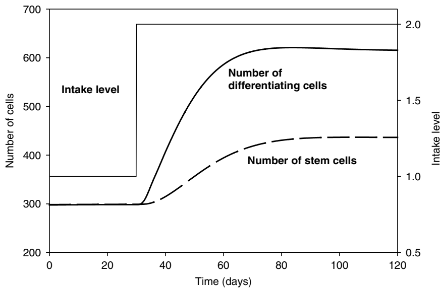
Fig. 22.3. The response predicted in the number of differentiating cells in the follicle bulb, N_{Diff} , and the number of stem cells in the follicle bulb, N_{Stem} , when the level of intake is doubled at 30 days. The predictions are made by solving Eqs (22.1) to (22.22) that define the cellular model.
