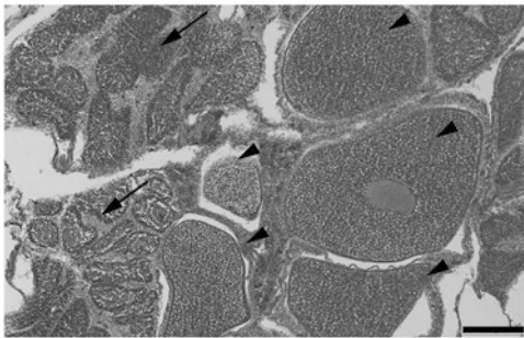
Fig. 8.3 Gamete bundles and gamete production in the coral Acropora tenuis . (a) Gamete bundles immediately after release during spawning. Each bundle comprises sperm surrounded by eggs. The arrow points to a wrapping membrane-like structure. Sperm and eggs separate after disruption of the membrane-like structure. (b) Hematoxylin-eosin stained coral fragment 7 days prior to a full moon in June. Arrowheads indicate eggs; arrows point to mature spermatozoa
