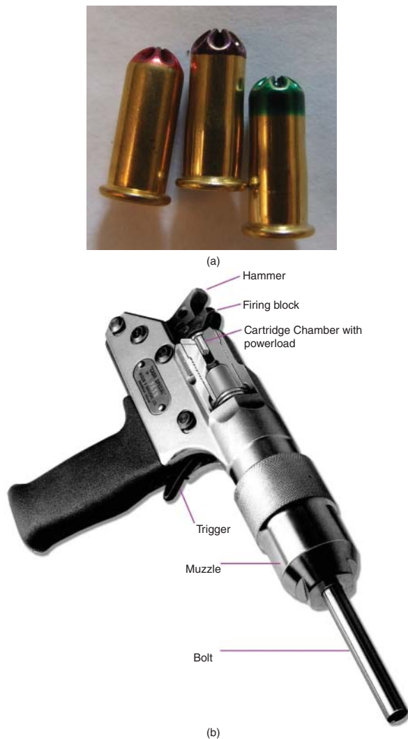
Figure 26.3 A CASH Special captive bolt gun (Reproduced courtesy of Accles & Shelvoke). (b) The bolt is shown extended for demonstration purposes. The inset (a) shows captive bolt cartridges in three power charges (from left to right: pink for calves, purple for heavy animals, green for bulls and very heavy animals).
