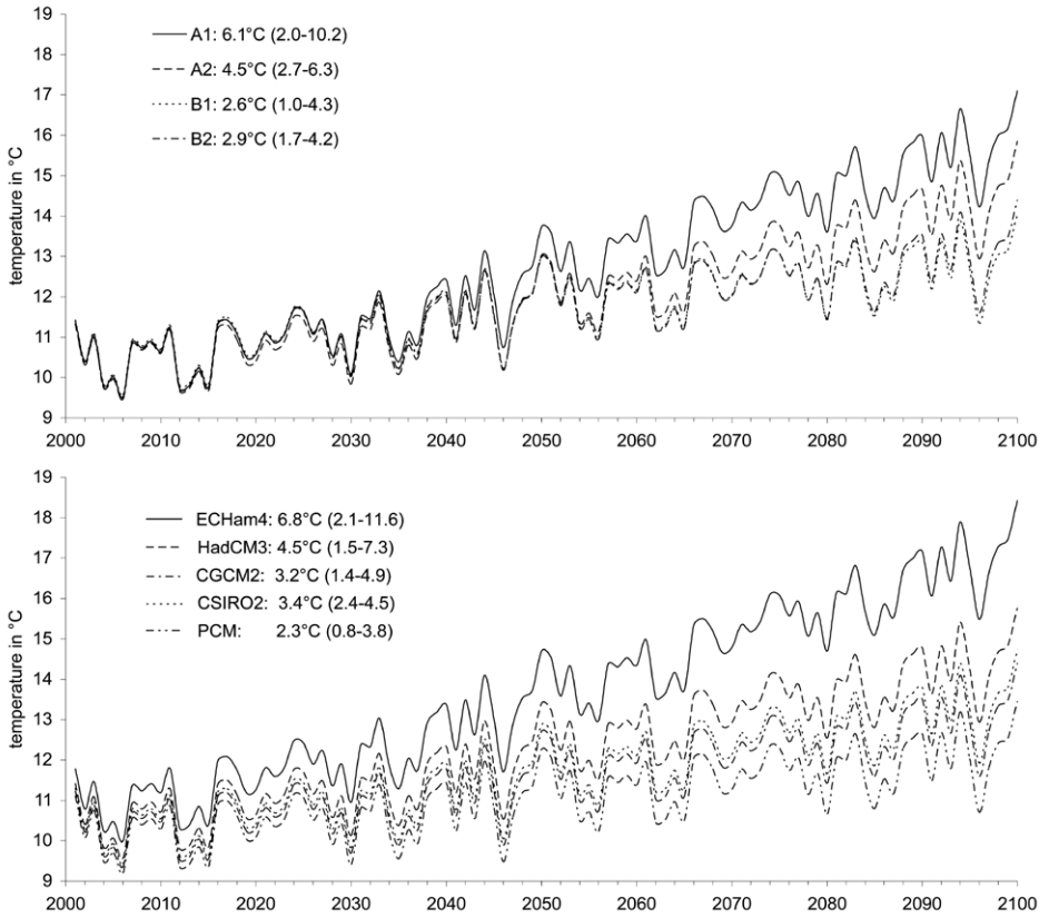
Figure 12. Time series of average annual temperature predictions for different emission scenarios (upper panel) and climate models (lower panel). Numbers in brackets denote the temperature range predicted by different climate models (upper panel) and different emission scenarios (lower panel). Grid-point Vienna, period 2001-2100.
