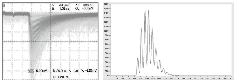
Fig. 3.22 Left: Oscilloscope picture of the signal from a G-APD (Hamamatsu 1-53-1A-1) recorded without an amplifier. Right: The corresponding pulse height spectrum. The mean number of photons in the recorded light flashes is about 2.5. Horizontal scale in arbitrary units
