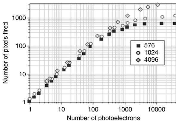
Fig. 3.23 Nonlinear response to a 40 ps laser light signal for G-APDs with different number of cells. Reprinted with permission from [59]
