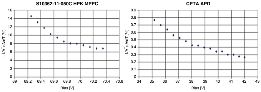
Fig. 3.25 Voltage coefficients k_V(V) of a G-APD from Hamamatsu ( left ) and from Photonique/CPTA ( right ) depending on the bias voltage at T=22 °C. Reprinted with permission from [60]
