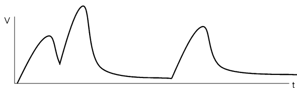
Fig. 5.12 Illustration of the signal pile up effect. The finite scintillator decay time dictates a signal charge integration time of typically at least two to three times the decay time, resulting in pulses with a relatively long trailing edge. In cases of high counting rates the possibility of detector pulses adding to the trailing edge of the preceding pulse increases, resulting in distorted pulse shapes
