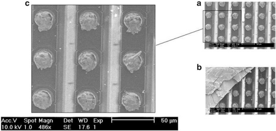
Fig. 2.9 (a) Scanning electron microscopy of a hybrid pixel detector, showing the indium bumps deposited with a pitch of 55 μm on the ASIC circuit. In (b), after hybridization, the sensor (a 1-mm thick CdTe detector) has been partially removed with a high strength force (scratched assembly). In (c) is a zoomed image of the bumps (courtesy of E. Manach, CEA-LIST, Saclay, France)
