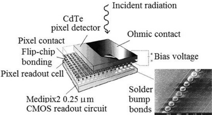
Fig. 2.22 MediSPECT is based on a hybrid pixel detector consisting of a CdTe pixel detector (1 mm thick, with ohmic contacts on both sides) and a Medipix2 readout ASIC with 55 \mu\text{m} square cells, as shown in this scheme
