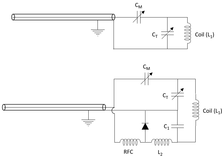
Fig. 7.12 Basic circuit diagrams for RF coil designs. The coil conductors which produces the RF field form the main inductance ( L_1 ) of the system while additional tuning (CT) and matching capacitors (CM) complete the resonant circuit and allow the coil to be tuned to the appropriate scanner frequency and matched to 50 \Omega impedance for optimum power transfer between the coil and rest of the system electronics. A more advanced coil design ( lower ) is also illustrated which could be used as a receive only coil within a larger volume transmit coil. Additional components in this design allow the coil to be detuned from the Larmor frequency via PIN diode switching. During RF excitation by a second coil a DC bias is supplied to the PIN diode via the RF choke (RFC) placing the additional inductance L_2 in parallel with tuning capacitor C_1 leading to an altered resonant frequency. During signal reception the PIN diode is off and inductance L_2 no longer contributes to the coil resonant frequency
