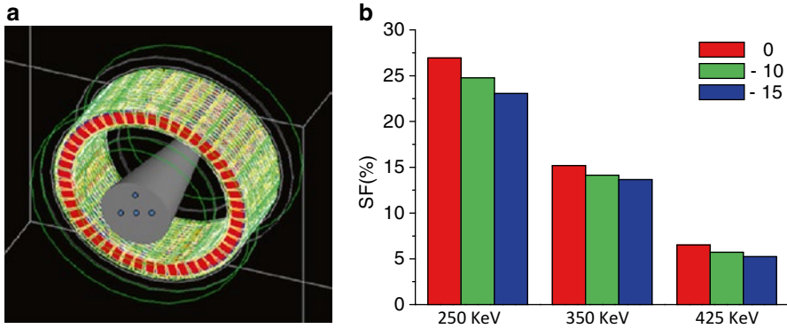
Fig. 17.3 Monte Carlo simulation model the LabPET™-8 small animal scanner ( left ). Representative example of the variation of the SF (in %) as a function of radial offsets for the cone-shaped phantom using a LET of 250, 350 and 425 keV for axial FOV mouse ( right )
