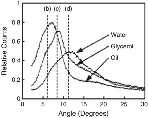
Fig. 6.10 X-ray scatter curves (more generally expressed as momentum transfer curves in which the X-ray wavelength is also accounted for) recorded from water, glycerol and oil which were illuminated by a pencil beam of 17.5 keV X-rays. Even though these curves were not corrected for the Compton scatter contribution, the different curves clearly allow discrimination of glycerol and oil which have very similar attenuation coefficients [43]
