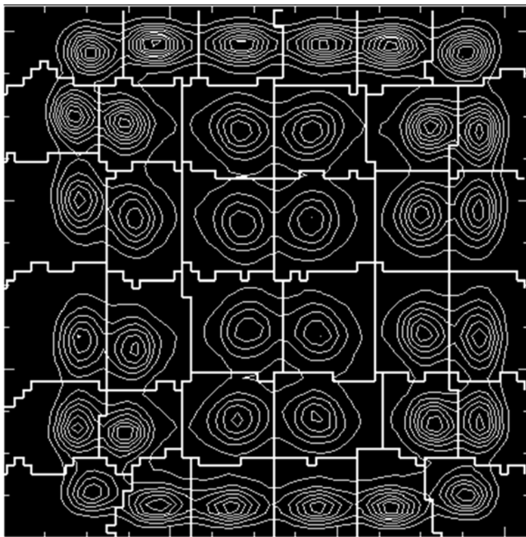
Fig. 1.4 A 2D block map of a 6×6 BGO crystal array viewed by four PMTs. The relative light output is indicated by the isocount curves. The “straight” lines indicate what regions will be assigned to each crystal position
