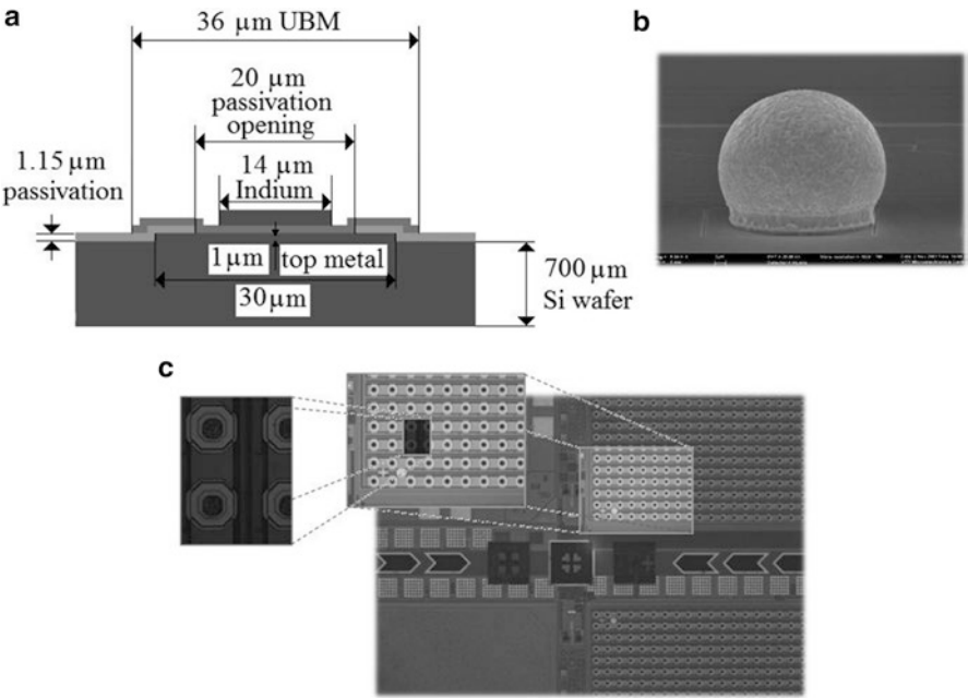
Fig. 2.8 Example of high-density indium bump-bonding: the Medipix2 hybrid pixel detector bump-bonded to a 700-μm thick silicon pixel detector with 55-μm-pitch pixels. (a) Scheme of the detector pixel, where a 36-μm square under-bump metallization (UBM) deposition is made at detector and ASIC substrates. (b) Scanning electron micrography of a 14 μm indium bump. (c) Patterning at the ASIC substrate showing, in successive magnifications, the pixel matrix array and the pixel bonding pads (courtesy of Z. Vykydal, IEAP, CTU, Prague)
