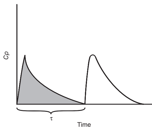
Fig. 12.2 Plasma concentration ( C_p )-versus-time profile after multiple extravascular drug administration, with no accumulation resulting in independent pharmacokinetics described by two single-dose profiles.
