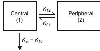
Fig. 8.15 Generalized open two-compartment pharmacokinetic model after intravenous administration with elimination ( K_{el} ) from the central compartment. K_{12} and K_{21} represent intercompartmental microrate constants.
