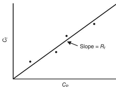
Fig. 11.2 Estimation of effective tissue:blood partition coefficients ( R_t ) at steady-state using a C_t -versus- C_p plot.
