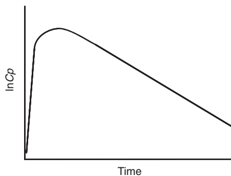
Fig. 8.9 Semilogarithmic plot of plasma concentration versus time with first-order absorption.
