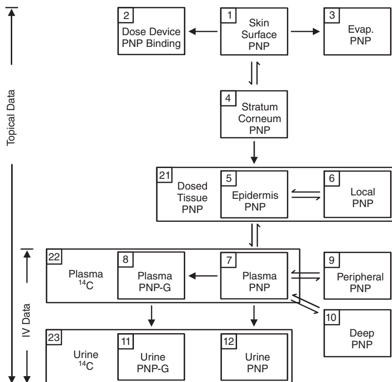
Fig. 8.25 Multicompartmental pharmacokinetic model used to study disposition of p -nitrophenol (PNP) after intravenous administration in pigs. These data were used to validate PNP parameters obtained from analysis described in Fig. 8.24.
