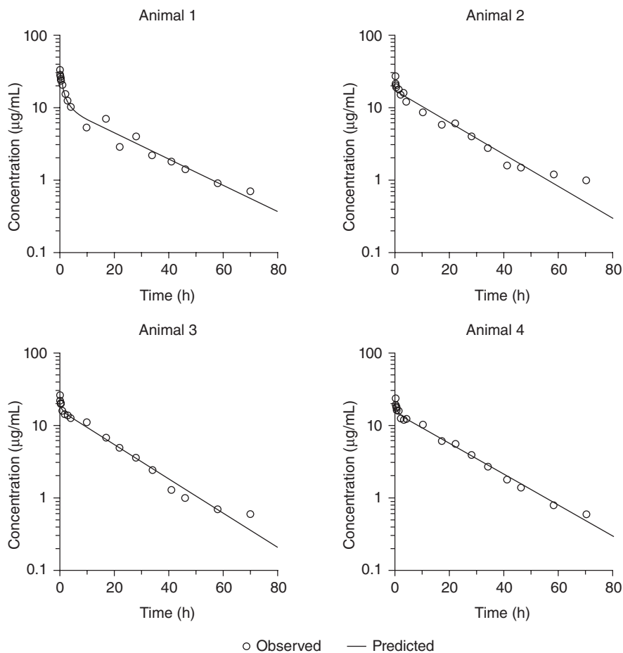
Fig. 14.7 Two-compartment, weighted (predicted -1 ) model fit. Note that in this case, there is not much change in the predictions.
