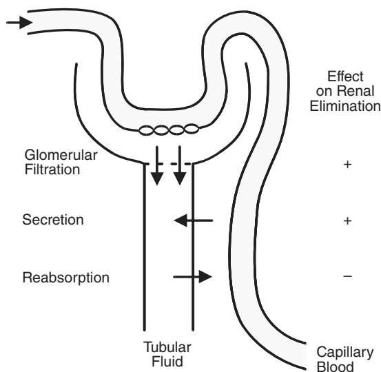
Fig. 6.2 Vectorial processes of nephron function and their net effect on overall renal drug elimination.
