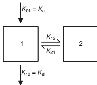
Fig. 8.18 Generalized open two-compartment pharmacokinetic model with first-order absorption ( K_{01} ) into and elimination ( K_{10} ) from the central compartment. K_{12} and K_{21} represent intercompartmental constants reflecting distribution.
