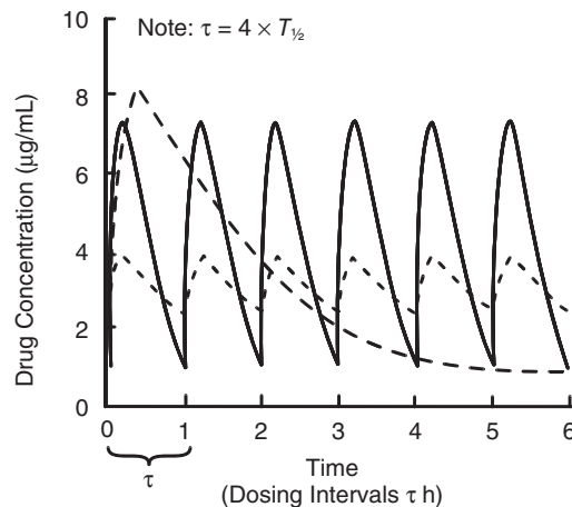
Fig. 17.3 Comparison of constant-dose (—) and constant-interval (----) regimens in renal failure ( Cl_c = one-sixth usual) with a normal dosage regimen (—) in a healthy patient. \tau is the dosage interval.
