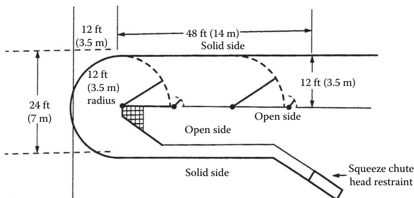
Figure 14.1 Cattle handling facility where the handler stands on the hatched area and works cattle from the crowd gate pivot. This takes advantage of the natural behavior of going back to where they came from.
