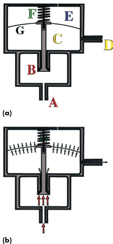
Figure 4.3 (a) Simplified diagrammatic section through reducing valve. (A) high pressure inlet, (B) high pressure chamber, (C) regulated pressure chamber, (D) regulated pressure outlet, (E) atmospheric pressure chamber, (F) spring. (b) Arrows represent forces: black arrows – forces due to high pressure gas, white arrows – forces due to regulated pressure gas, dashed arrows – forces due to atmospheric gas, dotted arrows – force due to spring.
