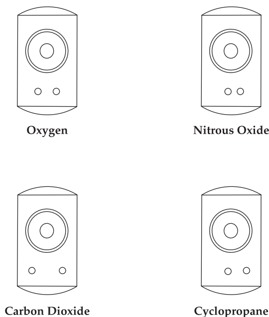
Figure 4.9 Pin index valve block system for small medical gas cylinders.
