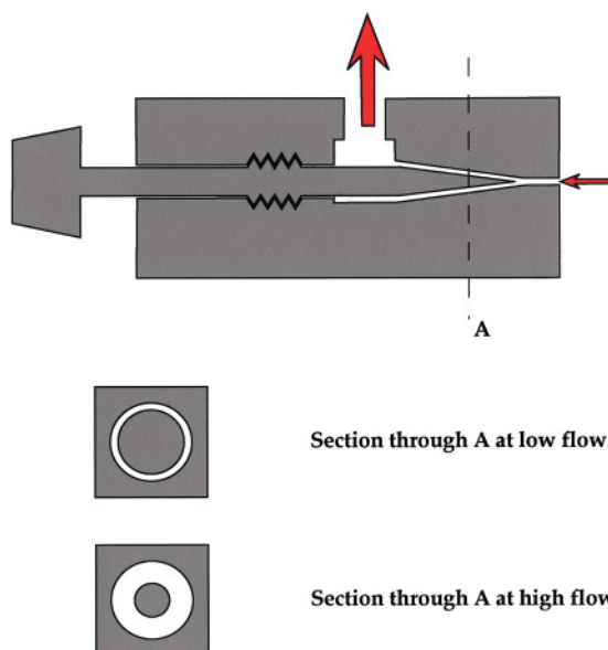
Figure 4.4 Diagrammatic section through needle valve. Turning the knob moves the needle into or out of its seat and alters the area through which gas may flow, thereby altering the resistance and so the flow of gas.
