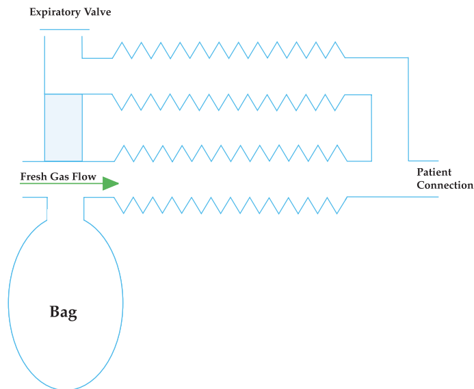
Figure 5.2 Parallel Lack breathing system.
