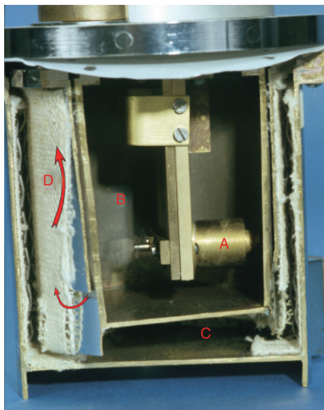
Figure 4.8 Cut-away of early Bowring Medical Engineering vaporiser. (A) thermostatic valve, (B) bypass chamber, (C) vaporisation chamber, (D) fibrous wicks.
