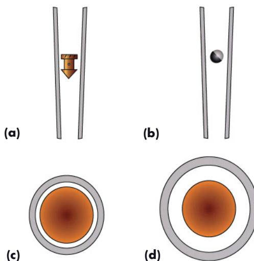
Figure 4.5 Diagrammatic representation of rotameter.
