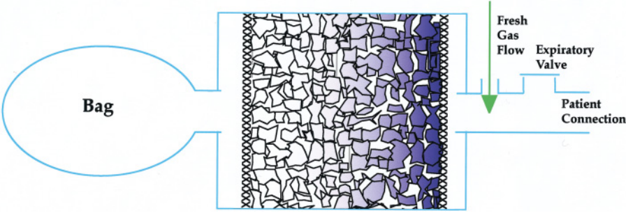
Figure 5.9 Water's canister (to-and-fro) breathing system.
