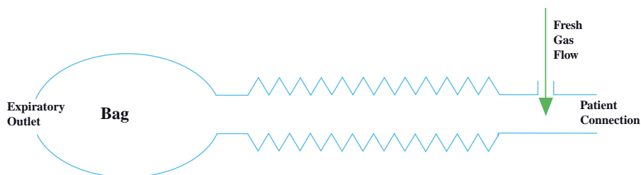
Figure 5.5 Jackson-Rees T-piece.
