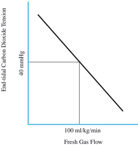
Figure 5.8 Changes in \text{PaCO}_2 with fresh gas flow using a Mapleson DEF system under IPPV. Graph of fresh gas flow against end-tidal carbon dioxide tension in a dog during IPPV ventilation using a Mapleson D, E or F breathing system (adapted from JFR Hird & F Carlucci, 1977). The use of the coaxial system to control the degree of rebreathing in the anaesthetised dog. Proc Ass Vet An G Br & Ir 7 .
