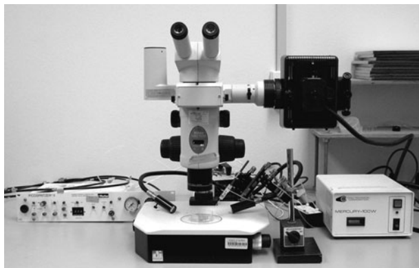
Fig. 16.3. The setup for microinjection. A picospritzer operated with a foot pedal (not shown) is at the left . A microscope used is shown; in this case a fluorescence microscope with 15× eyepieces, although a non-fluorescence microscope with 40× objective and 10× eyepieces is adequate. Fiber optics are adjusted so that the light reflects off eggs in the Petri dish on the stage of the microscope. The micromanipulator is adjusted so that the needle is at a 45° angle.
