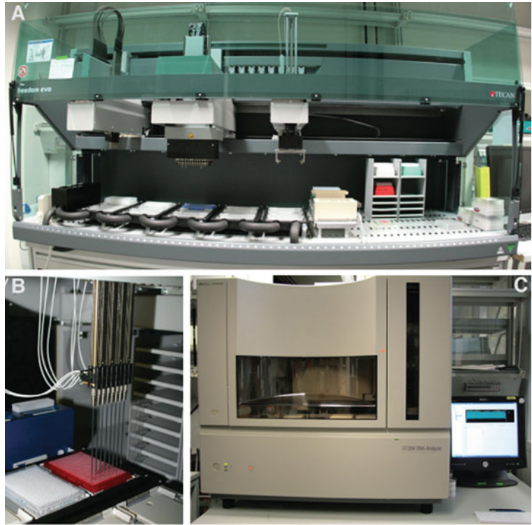
Fig. 19.5. Liquid handling setup of the Dresden TILLING facility. (a) The setup contains a liquid handling pipetting station (TECAN Freedom) that allows low volume (b) as well as multichannel pipetting (96-well liquid handling tool). All liquid handling, PCR amplification, and sequencing steps are performed in 384-well format (b). (c) 384-well plates are sequenced on an AB3730XL DNA sequencer.
