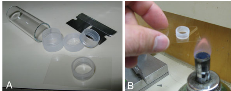
Fig. 2.3. Constructing an inverted-microscope observation chamber. (a) Nylon cap from shell vial is cut with razor. Cylinder is dipped briefly in molten wax and placed on clean coverslip. (b) Coverslip is briefly flamed to reheat wax which seals lip of cap to the glass. The wax seal is suitable for all aqueous media as well as Murray Clear.
