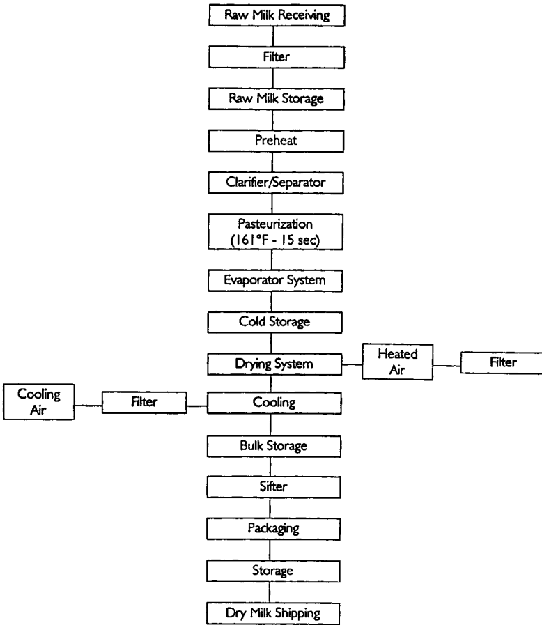
Figure 3 Processing scheme for dry milk.
