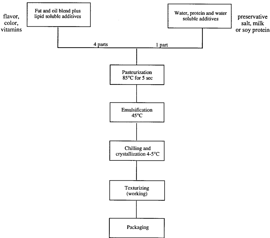
Figure 13 Manufacturing flow diagram for margarine-type products.
