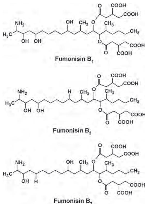
FIG. 3 Chemical structures of fumonisins.
