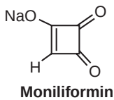
FIG. 4 Chemical structure of moniliformin.
