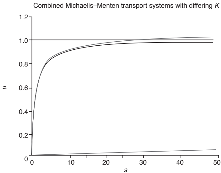
Fig. 9.9. Combined Michaelis-Menten transport systems operating in parallel. Values used are given in equation 7.
