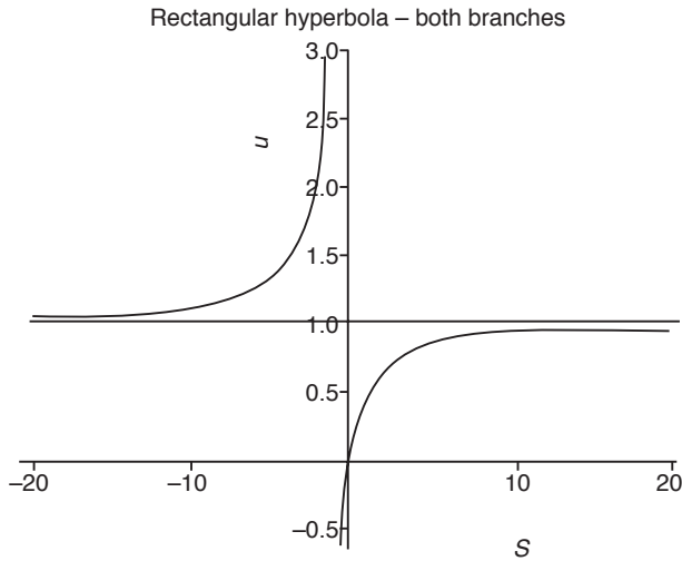
Fig. 9.2. Rectangular hyperbola used to describe Michaelis–Menten kinetics ( S > 0 ) but also showing the non-realistic but mathematically important second branch for S < -K_m .
