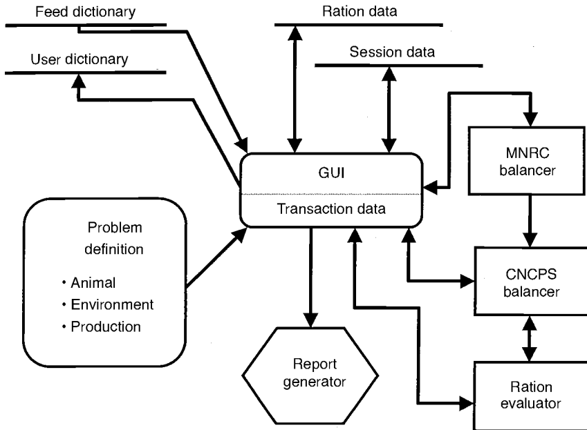
Fig. 28.2. An architectural overview of CPM-Dairy. Regular boxes represent processing modules, rounded boxes represent data display and data collection modules and the hexagon represents a data output module. Horizontal lines represent data stores, and the arrow lines represent data exchange. MNRC, modified National Research Council.
