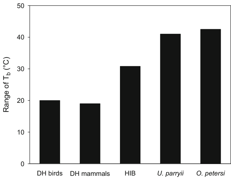
Fig. 5.7 The range of T_b for average avian and mammalian daily heterotherms (DH), mammalian hibernators (HIB) and two extreme values for arctic ground squirrels ( Uroditellus parryii ) and a desert bat ( Ozimops petersi ). Data from Barnes (1989), Bondarenco et al. (2014), Ruf and Geiser (2015)
