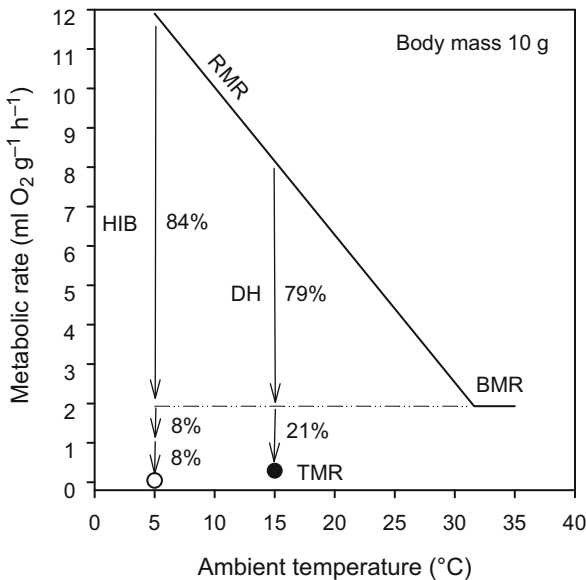
Fig. 5.13 Metabolic rate (MR) reduction during torpor entry vs ambient temperature (T a ) for a 10-g hibernator (HIB) and daily heterotherm (DH). The arrows indicate the fall due to de-activation of normothermic thermoregulation (RMR to BMR) near the T a below which thermoregulation is activated during torpor, the % values show by how much the MR is reduced from RMR to BMR (84% HIB, 79% DH). For DH (filled circle) it is assumed that the fall of MR below BMR to TMR is entirely due to the fall of T b (DH 21%), for HIB (circle) it is assumed that the fall of MR below BMR is due to half physiological inhibition and half the fall of T b (8% and 8% each). Data from Bradley and Deavers (1980), Riek and Geiser (2013), Ruf and Geiser (2015)
