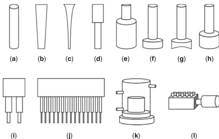
Figure 13.3 Horn shapes: a) cylindrical, b) conical, c) exponential, d) stepped, e) full wave, f) half wave, g) half wave with an opening, h) half wave booster, i) dual probe, j) multi probe, k) cup horn, and l) horn for vials.
