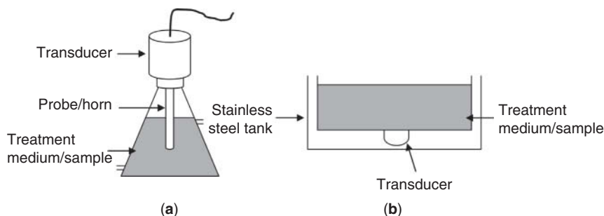
Figure 13.2 (a) ultrasound horn; (b) ultrasound bath.
