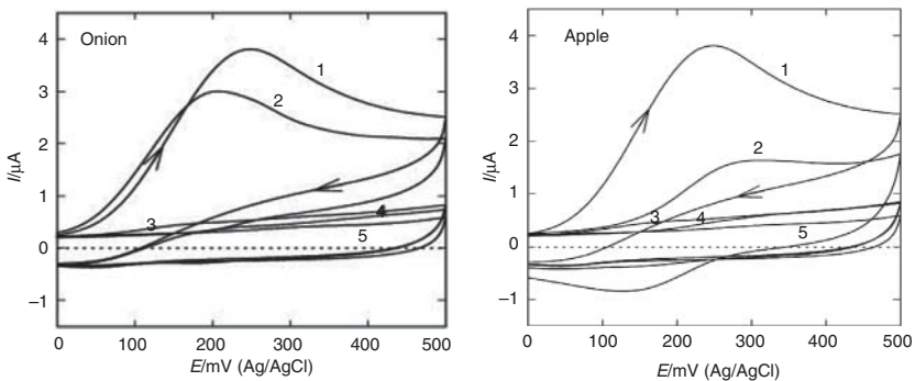
Figure 5.2 Cyclic voltammograms of ascorbic acid in the presence of onion or apple fibre prepared using an aqueous method. Curve: 1, Ascorbic acid before incubation (pH 6.5, 37°C); 2, Antioxidant plus onion or apple fibres after incubation; 3, Ascorbic acid after incubation; 4, onion or apple fibres after incubation; 5, Buffer solution background (HEPES 15 mM).
