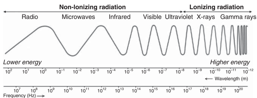
Figure 4.2 Electromagnetic spectrum.
