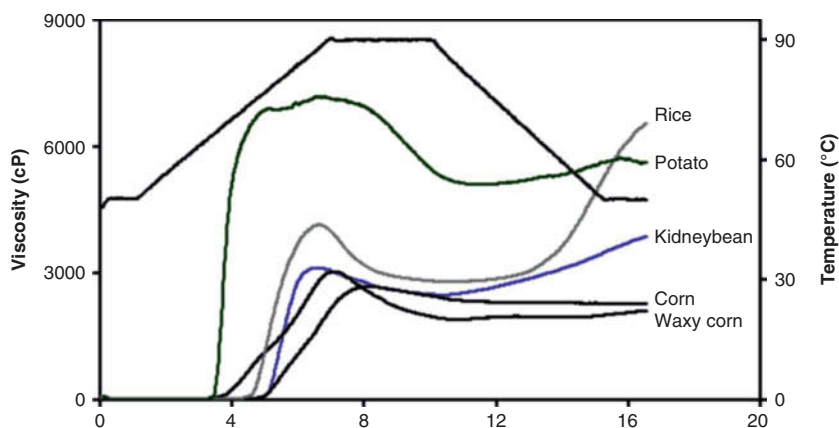
Figure 2.2 Pasting profiles of different starches measured using RVA.
