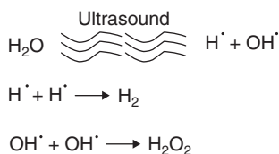
Figure 13.1 Water sonolysis and radicals combinations.
