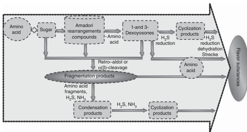
Figure 9.1 Schematic diagram of different pathways of Maillard reaction.
