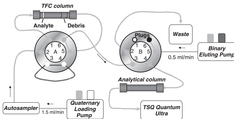
Figure 4.5 Schematic representation of the loading step in an Aria TLX-2 system. The sample is introduced into the system by an autosampler and a loading pump. The system also involves a solvent holding loop connected to valve A. This loop contains a solvent mixture strong enough to elute the analytes from the TurboFlow column (TFC) into the analytical column (transfer step). An eluting pump delivers a mixture of solvents and enables a normal chromatographic separation and detection. (Adapted from Stolker et al. 146 with permission from Springer; copyright 2010.)
