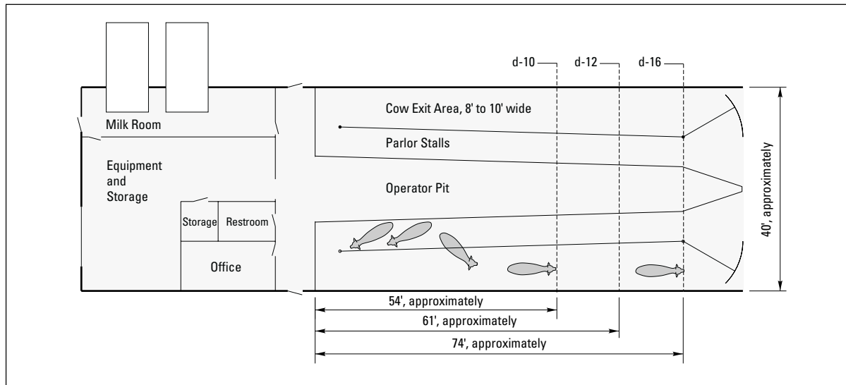
Figure 5-6. Rapid-exit parlor.
