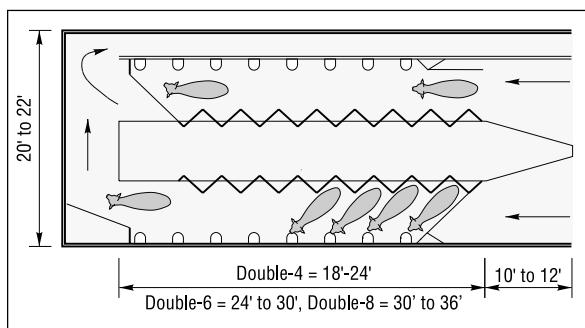
Figure 5-3. Double-8 herringbone parlor.
