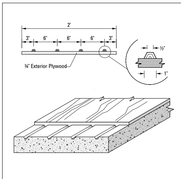
Figure 4-7. Homemade beveled groover.
