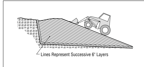
Figure 9-1. Filling horizontal silos.
