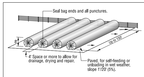
Figure 9-3. Horizontal plastic bags.
