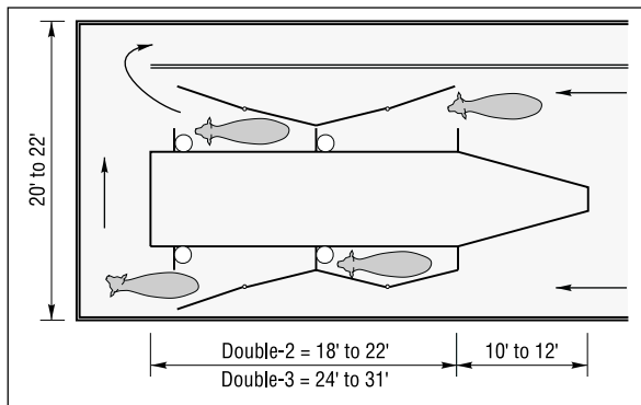
Figure 5-2. Double-2 side-opening parlor.
