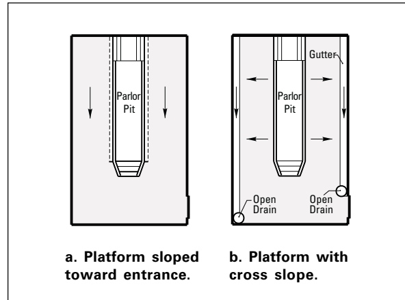
Figure 5-17. Milking platform drain system.
