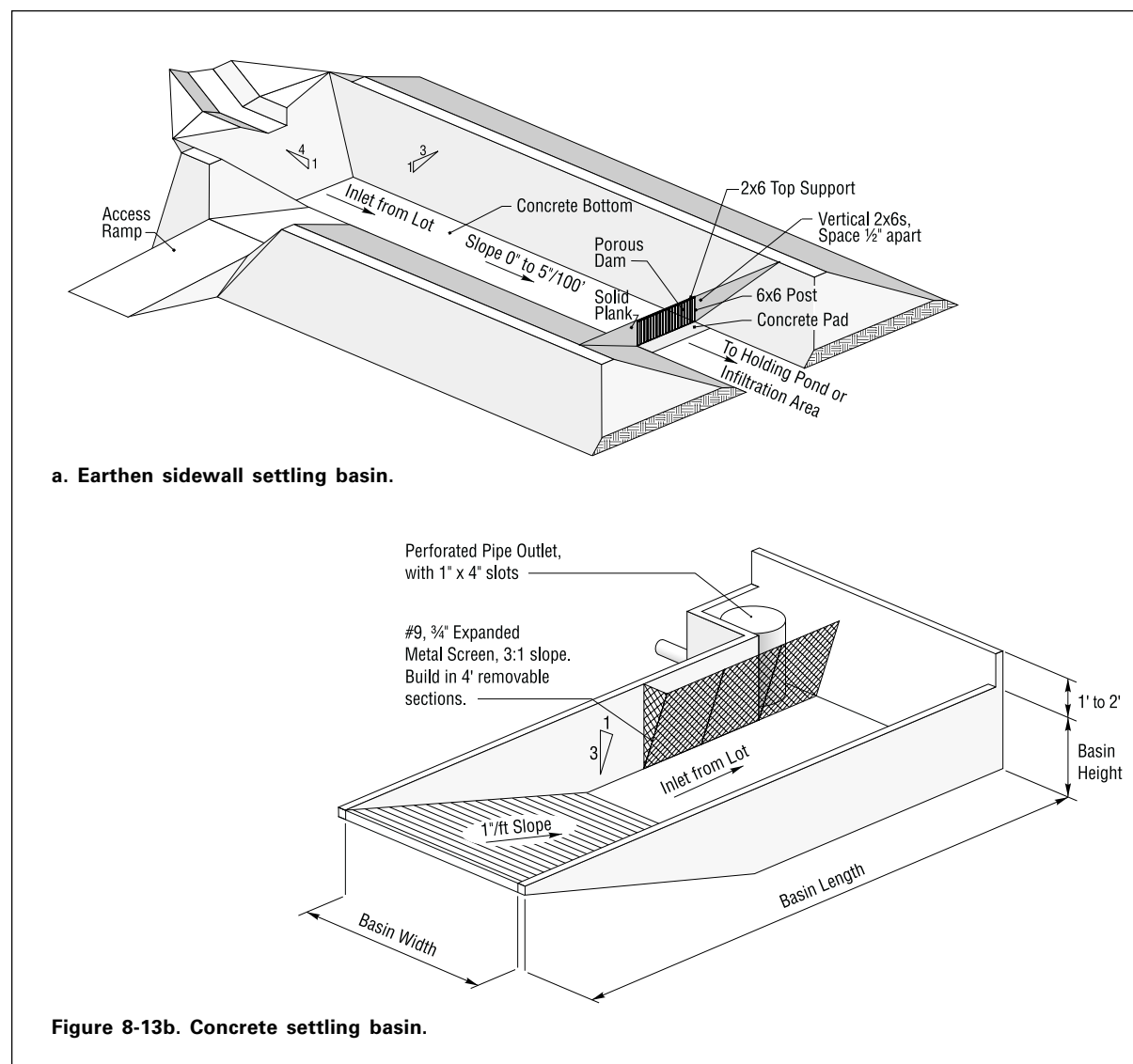
Figure 8-13. Settling basins.
