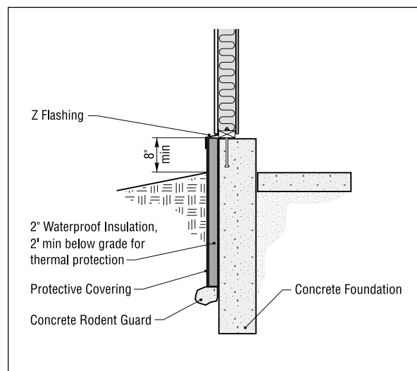
Figure 7-14. Insulating foundations.
