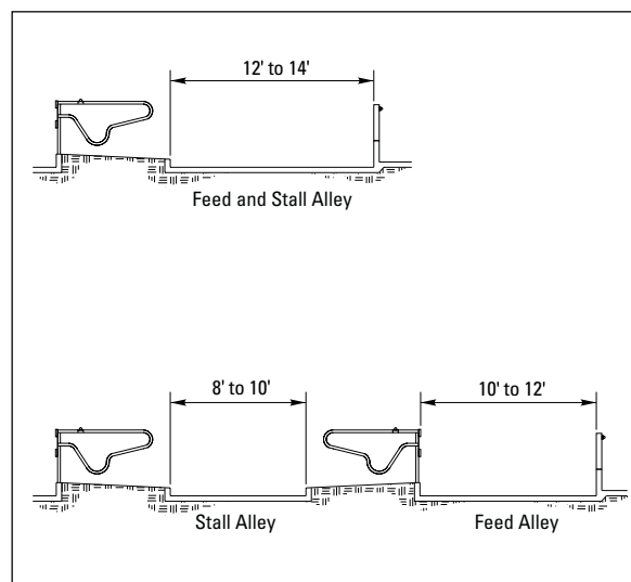
Figure 4-9. Alley types.
