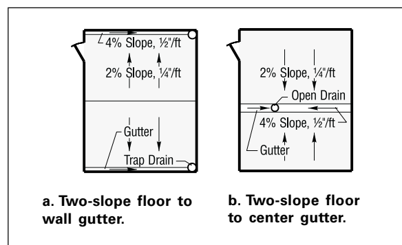
Figure 5-16. Milk room floor slopes. Slope floors a minimum of 2% (1/4"/ft).
