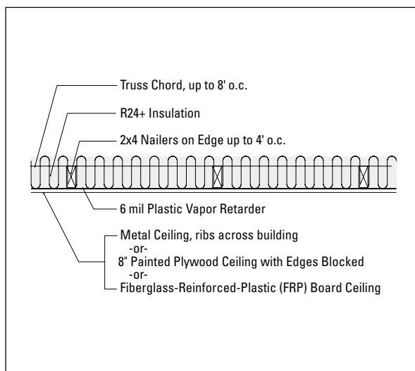
Figure 7-12. Insulating ceilings.
