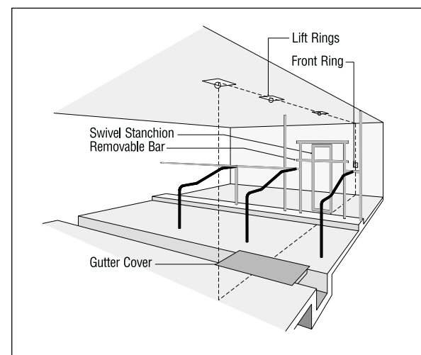
Figure 6-3. Treatment stall.
