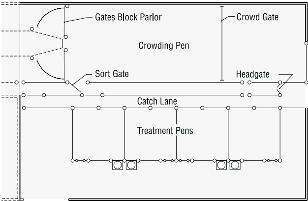
b. Gates block parlor entrance. Use gates to block parlor entrance. Holding area acts as a crowding pen to direct cows into the handling lane. A headgate can be used to restrain cows, or they can be directed into a separate pen.
