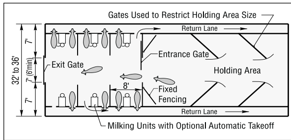
Figure 5-1. Flat-barn parlor.
