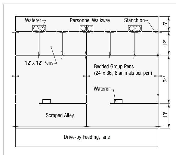
Figure 4-19. Barn with bedded group and individual pens.
