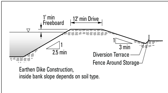
Figure 8-14. Holding pond.
