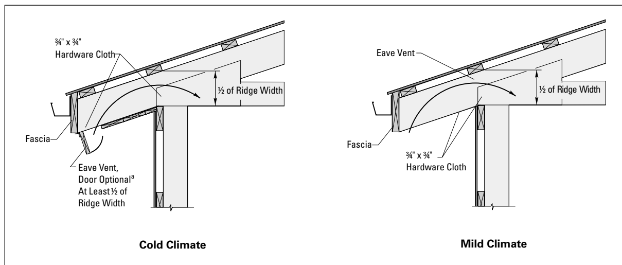
Figure 7-6. Eave openings.
