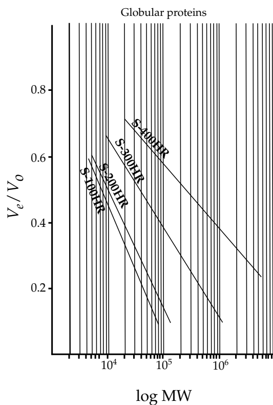
FIGURE 7.6 V_e/V_o versus log MW for Sephacryl resins
