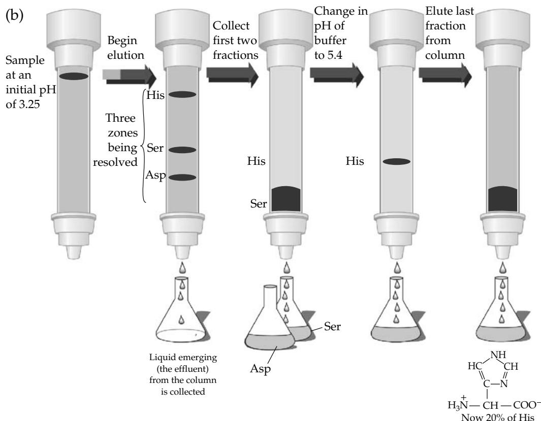
FIGURE 5.3 Elution of amino acids with ion-exchange chromatography
