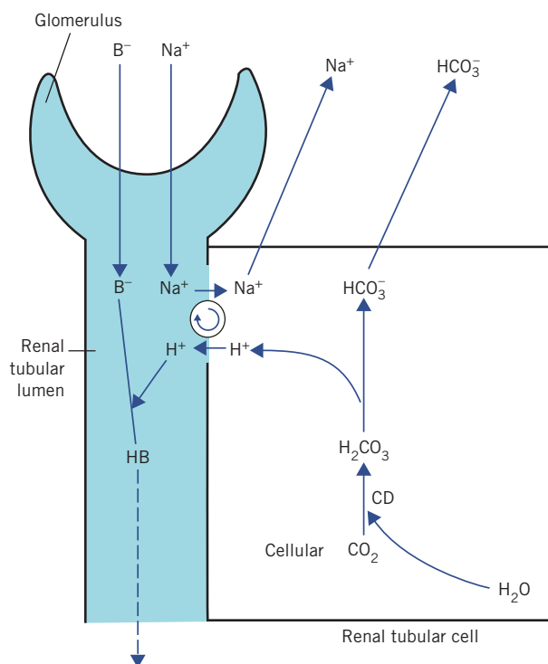
Figure 4.3 Net generation of bicarbonate by renal tubular cells with excretion of hydrogen ions. B^- , non-bicarbonate base; CD, carbonate dehydratase.
