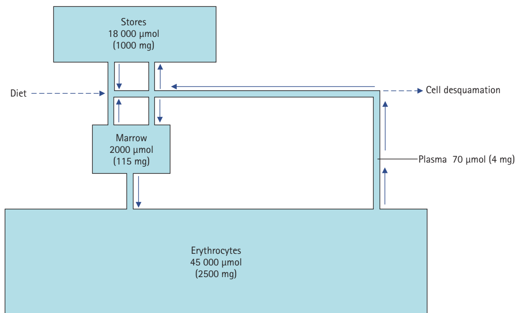
Figure 21.3 Body iron compartments.
