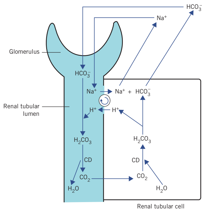
Figure 4.2 Normal reabsorption of filtered bicarbonate from the renal tubules. CD, carbonate dehydratase.
