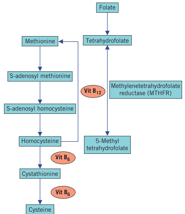
Figure 15.2 Diagram showing simplified pathways of homocysteine metabolism.
