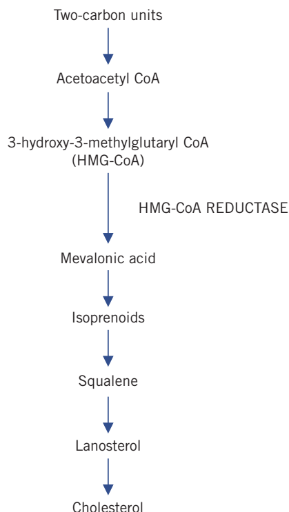
Figure 13.4 Summary of pathways of cholesterol synthesis. CoA, coenzyme A. Reproduced with kind permission from Candlish JK and Crook M. Notes on Clinical Biochemistry . Singapore: World Scientific Publishing, 1993.
