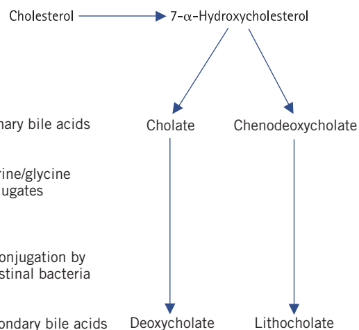
Figure 17.5 Synthesis of bile acids in the liver and their conversion to secondary bile salts in the intestine.
