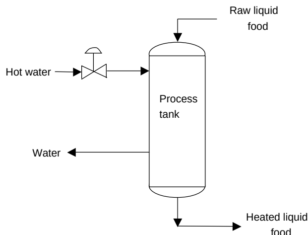
Figure 10.3 A process tank to heat liquid food using hot water.
