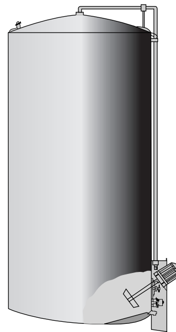
Figure 10.6 A tank with a propeller agitator. (Source: Dairy Processing Handbook , Tetra Pak.)
