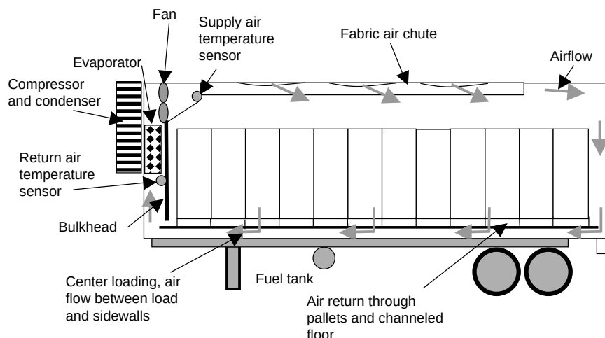
Figure 10.15 Airflow in a refrigerated trailer.
