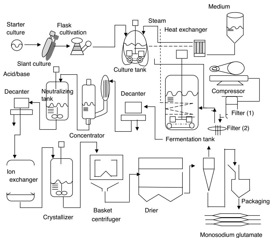
Figure 5.7 Flow diagram of the industrial production of glutamate.
