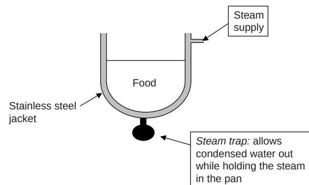
Figure 9.13 Jacketed pan.
