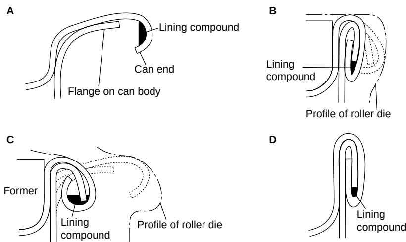
Figure 11.4 Double seaming of metal ends onto metal containers: A, end and body are brought together; B, first seaming operation; C, second seaming operation; D, section through final seam. (Copyright 2006. From Food Packaging Principles & Practice by G.L. Robertson. Reproduced by permission of Routledge/Taylor & Francis Group, LLC.)
