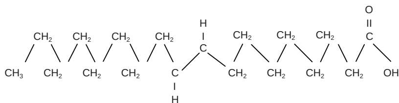
Figure 12.3 trans Acid.
