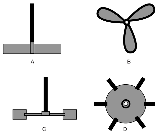
Figure 9.26 Devices for the mixing of low viscosity liquids: A a paddle; B a three-blade propeller; C (side view) and D (top view) a six-blade turbine.
