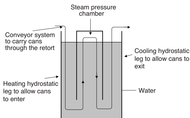
Figure 9.33 Hydrostatic retort.
