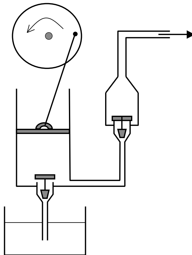
Figure 9.11 Reciprocating piston pump.
