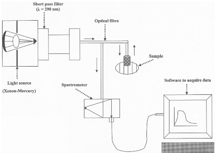
Fig. 14.1 Evaluation of raw meat tenderness with spectrofluorometry (Frenicia et al. , 2002).
