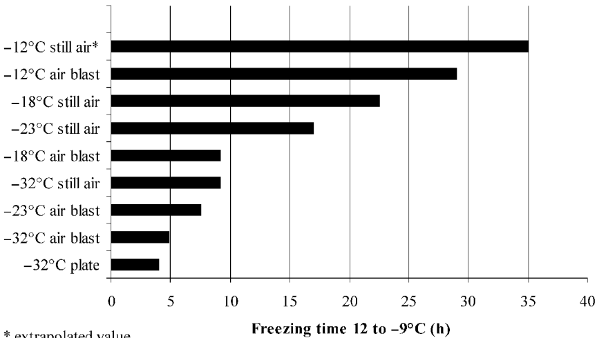
Fig. 8.2 Freezing time of 2.3 kg chicken carcasses under different freezing regimes (DuBois et al. , 1942).
