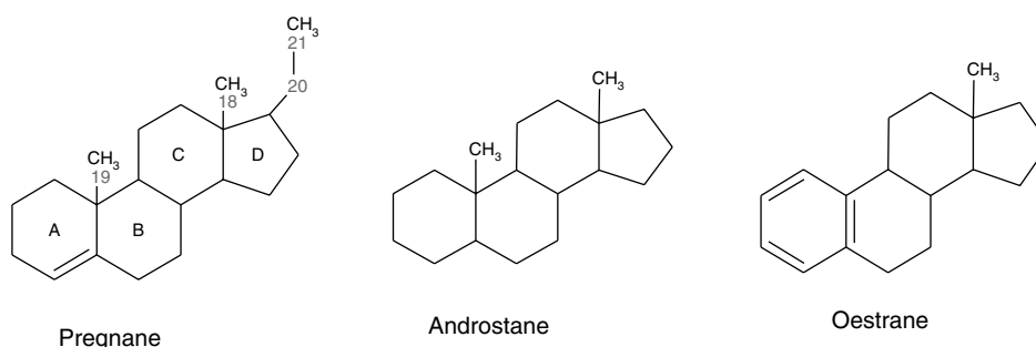
Fig. 2.32. Pregnane, androstane and oestrane steroid structures. Pregnane (C21) indicates a steroid structure with methyl groups at C13 and C10 and a two-carbon-atom side chain attached at the C17 position. Androstane (C19) indicates a steroid structure with methyl groups at both the C13 and C10 positions. Oestrane (C18) indicates a steroid structure with a methyl group attached at C13 and an aromatic A ring.
