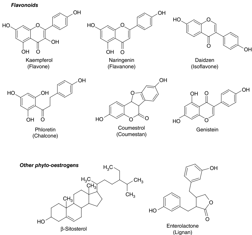
Fig. 6.26. Oestrogenic and anti-oestrogenic compounds from plants.
