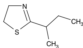
2- sec -Butyldihydrothiazole
