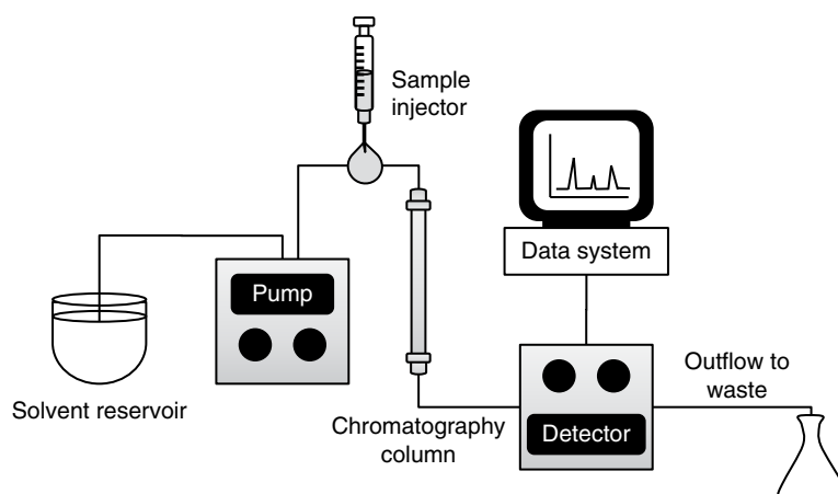
Fig. 2.27. Typical chromatography system.
