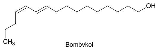
Fig. 6.8. Sex pheromone of the female silkworm.
