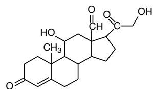
Aldosterone
