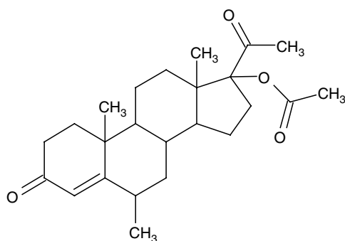
17-Acetoxy-6-methylprogesterone (MAP)
