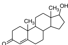
Testosterone
