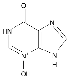
Hypoxanthine-3N-oxide
