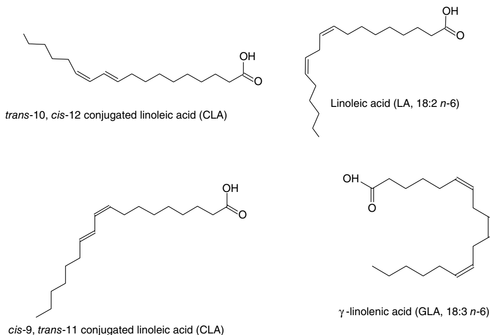
Fig. 3.31. Structures of linoleic acid, conjugated linoleic acid and \gamma -linolenic acid.
