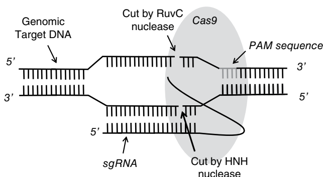
Fig. 2.46. The CRISPR/Cas system for gene editing. Site-specific DNA cleavage of the genomic target sequence by nuclease Cas9 is directed by a single-guide RNA (sgRNA) when a protospacer-adjacent motif (PAM) is present on the opposite strand.
