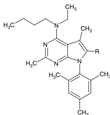
Fig. 6.18. Structure of CRHR1 receptor antagonist. For CP 154,526, R = H; for antalarmin, R = CH 3 .
