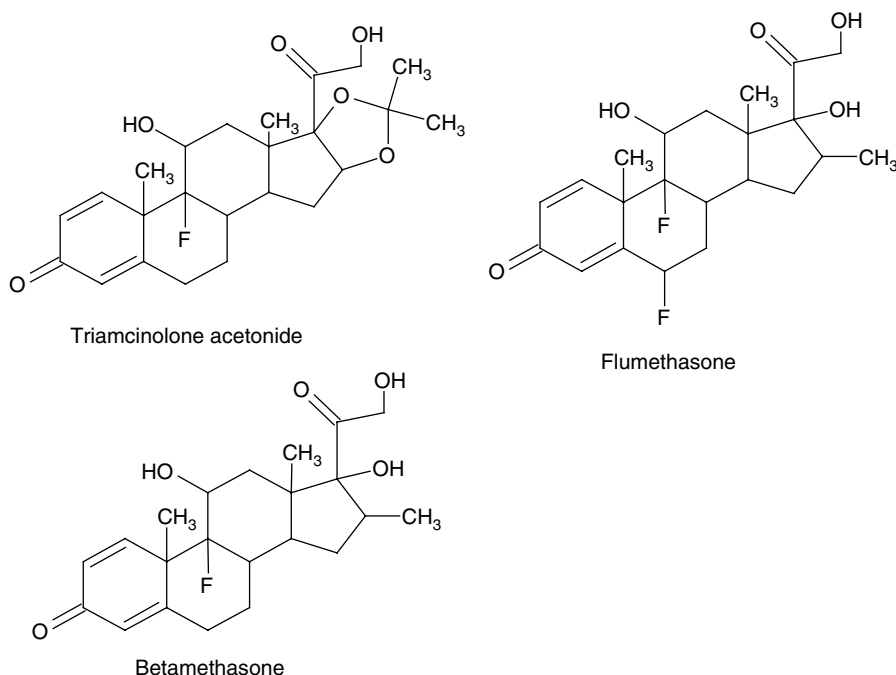
Fig. 5.8. Structures of some synthetic corticosteroids.
