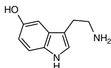
Serotonin
