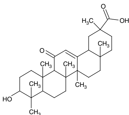
Glycyrrhetic acid
