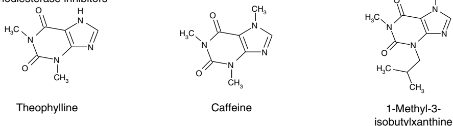
Fig. 1.31. cAMP and its analogues and phosphodiesterase inhibitors.
