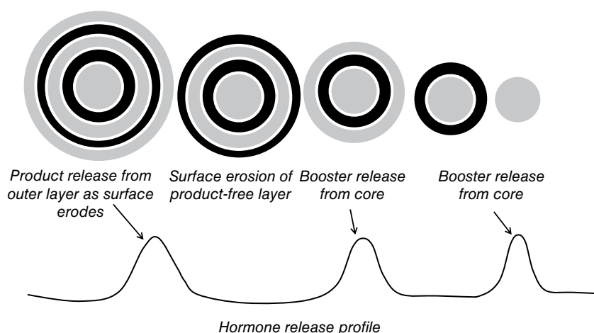
Fig. 2.43. Surface eroding system for pulsatile release of hormones.
