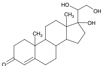
17 \alpha ,20 \beta ,21-tri-hydroxy-4-pregnen-3-one
