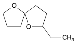
Spruce dark beetle pheromone (Chalcogran)
