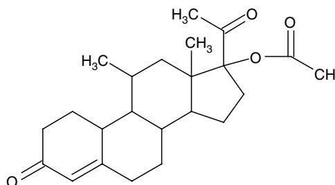
Norgestomet
