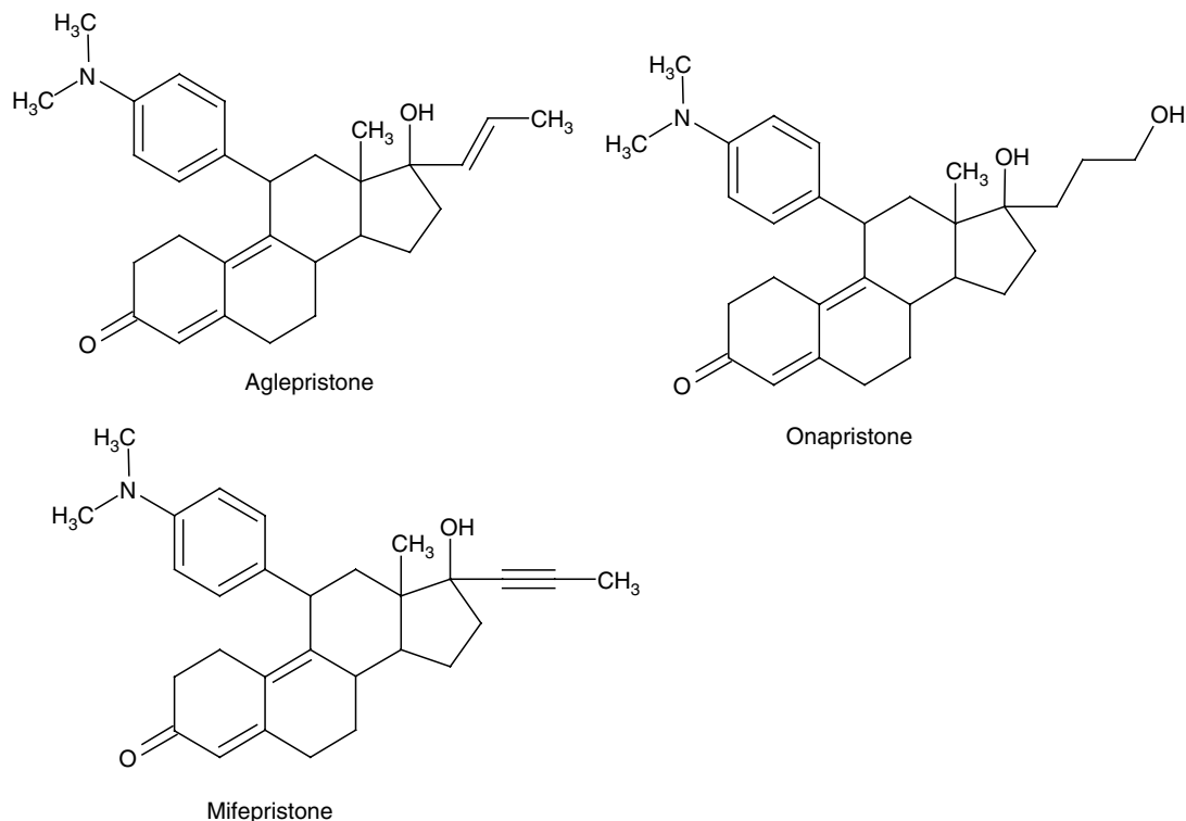
Fig. 5.9. Structures of some synthetic anti-progestogens.
