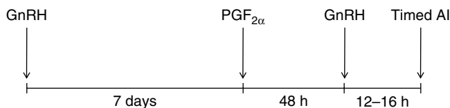
Fig. 5.13. Ovsynch® protocol for oestrus synchronization.
