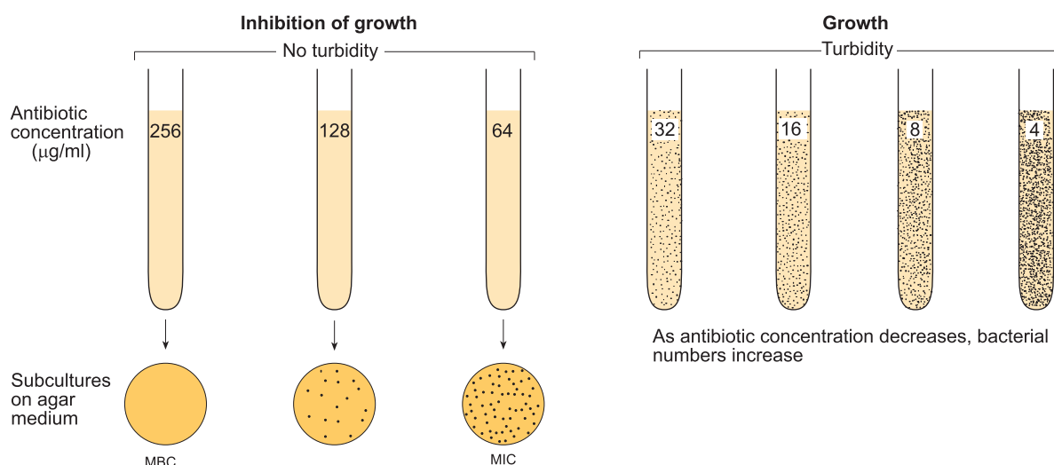
Dilution method for determination of the minimal inhibitory concentration (MIC) and the minimal bactericidal concentration (MBC) of an antibiotic for a test bacterium
