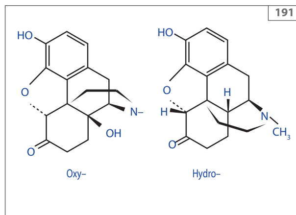
Fig. 191 Structure of oxymorphone and hydromorphone.
