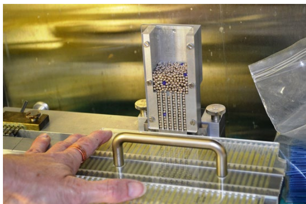
Figure 78.1 Sealing of straws using metal beads.
