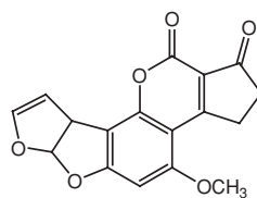
Aflatoxin B 1
