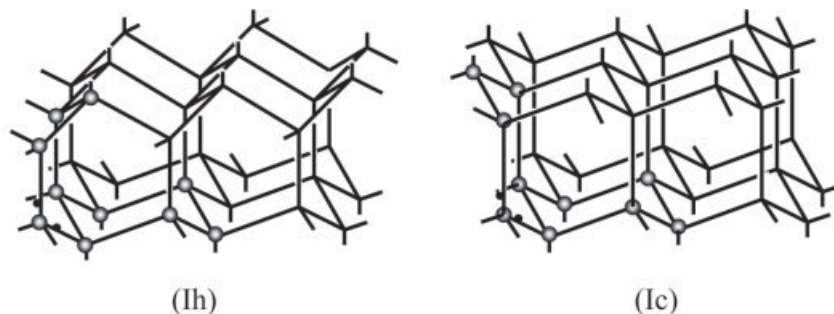
Figure 5.5. The crystal structures of ice hexagonalice (Ih) and cubic ice (Ic). Oxygen atoms are placed in two rings in each to point out their subtle difference. Each line represents a hydrogen bond O—H—O, and the H atoms are randomly distributed such that on average, every oxygen atom has two O—H bonds of 100 pm. The O—H—O distance is 275 pm. The idealized tetrahedral bond angles around oxygen are 109.5°.
