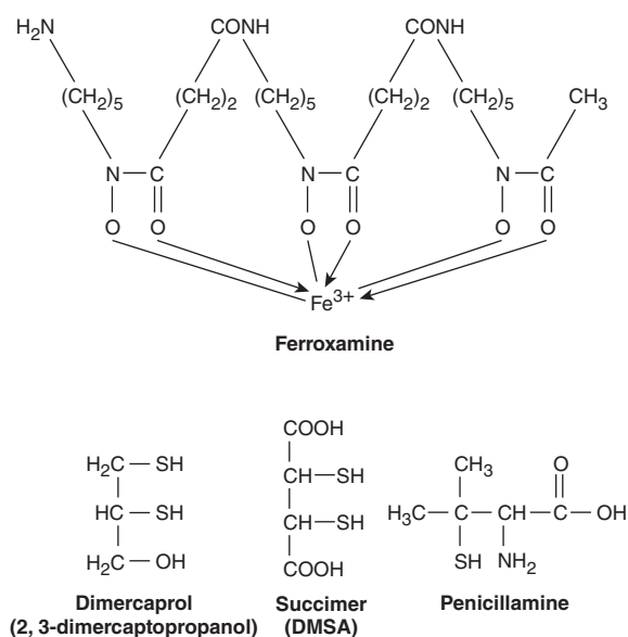
FIGURE 57–3 Chemical structures of several chelators.
