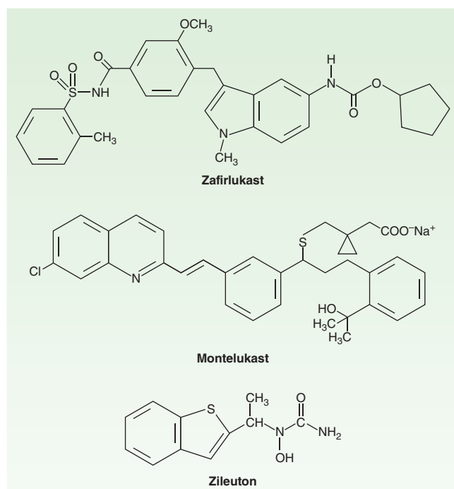
FIGURE 20-6 Structures of leukotriene receptor antagonists (montelukast, zafirlukast) and of the 5-lipoxygenase inhibitor (zileuton).
