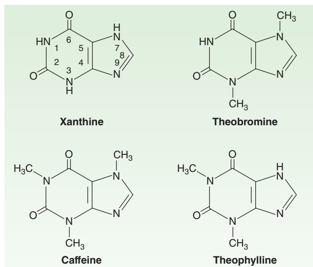
FIGURE 20–4 Structures of theophylline and other methylxanthines.
