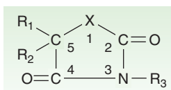
FIGURE 24-3 Antiseizure heterocyclic ring structure. The X varies as follows: hydantoin derivatives, -N- ; barbiturates, -C-N- ; oxazolidinediones, -O- ; succinimides, -C- ; acetylureas, -NH_2 (N connected to C_2 ). R_1 , R_2 , and R_3 vary within each subgroup.
