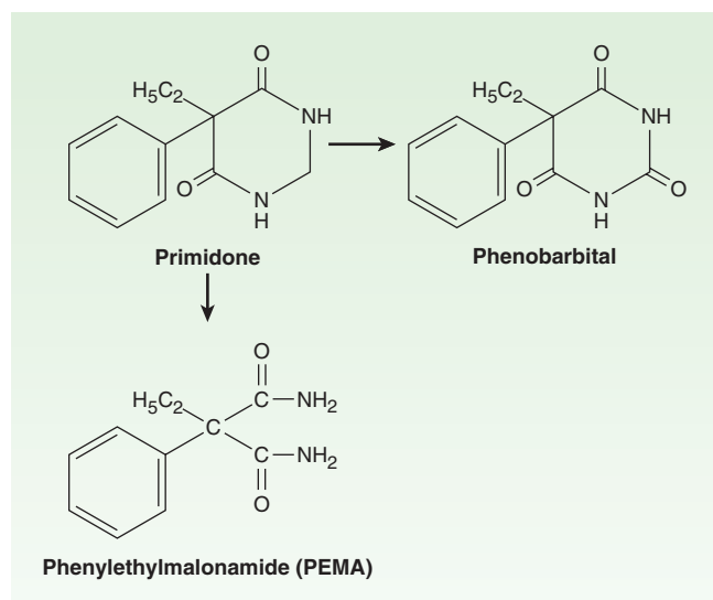
FIGURE 24–6 Primidone and its active metabolites.
