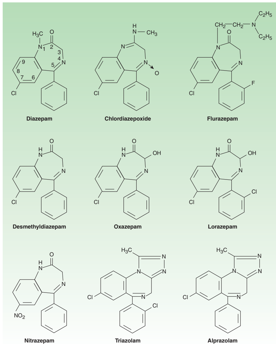
FIGURE 22-2 Chemical structures of benzodiazepines.
