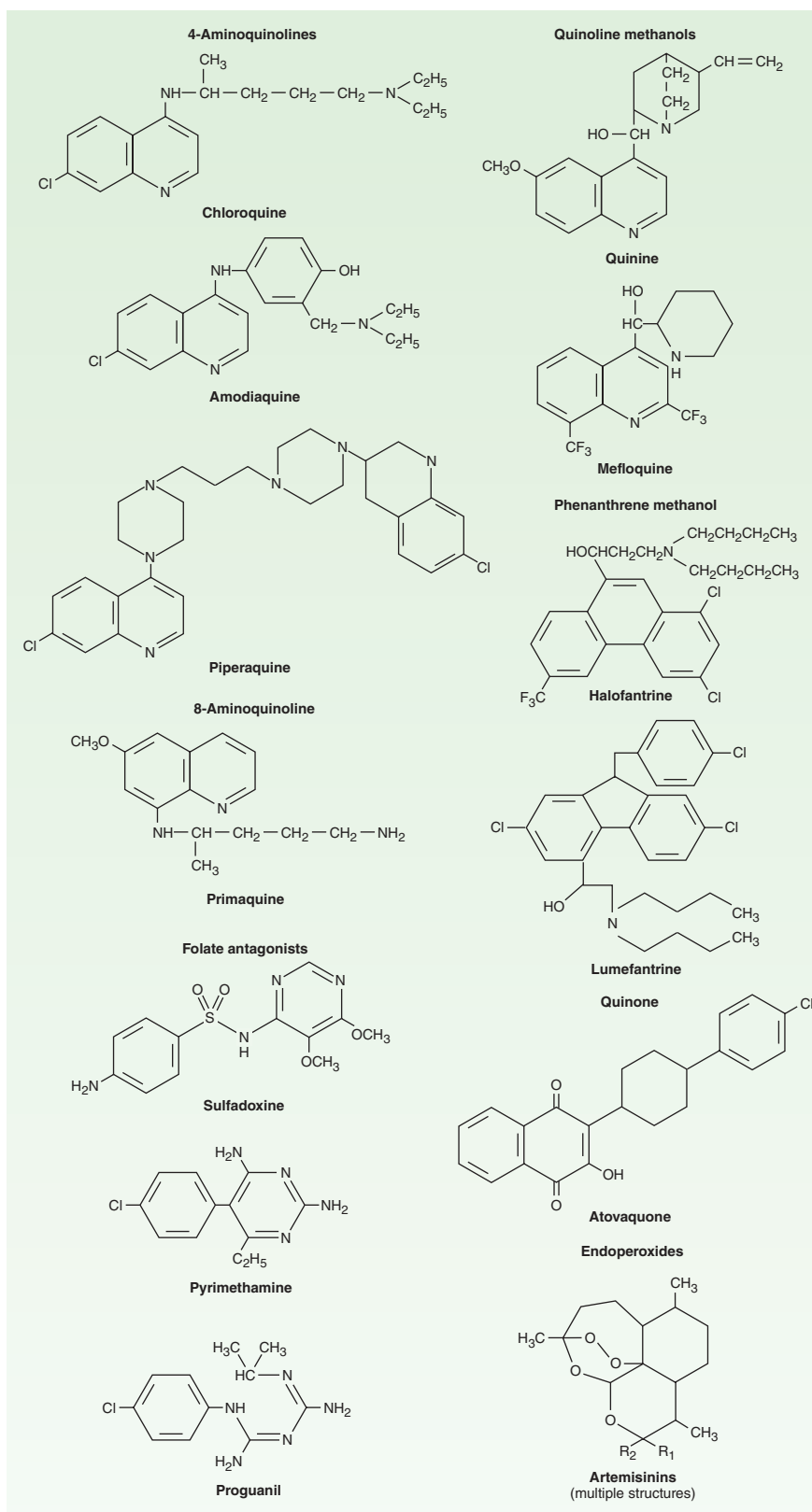
FIGURE 52-2 Structural formulas of some antimalarial drugs.
