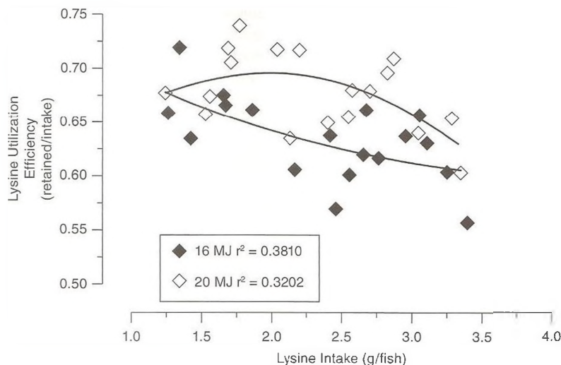
FIGURE 5-3 Effect of lysine and DE content of the diet (3.82 vs. 4.78 Mcal DE or 16 or 20 MJ DE/kg) on efficiency of lysine utilization of rainbow trout ( Oncorhynchus mykiss ) (Encarnação et al., 2004).
