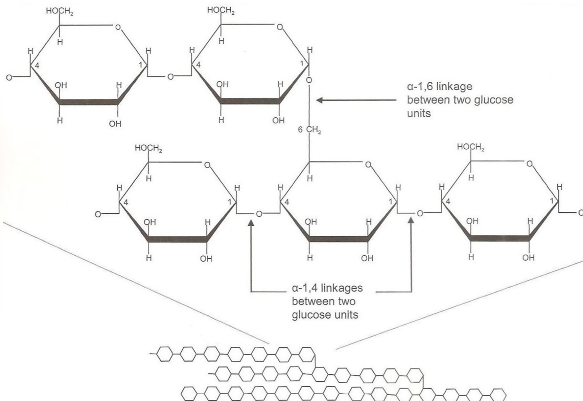
FIGURE 7-4 Structure of amylopectin.
