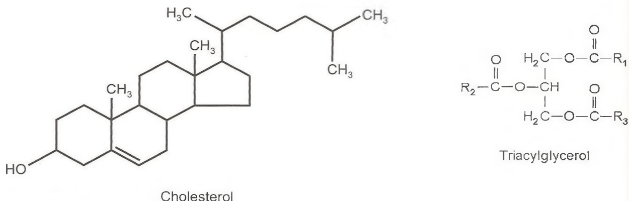
FIGURE 6-3 The structures of cholesterol and triacylglycerol.
