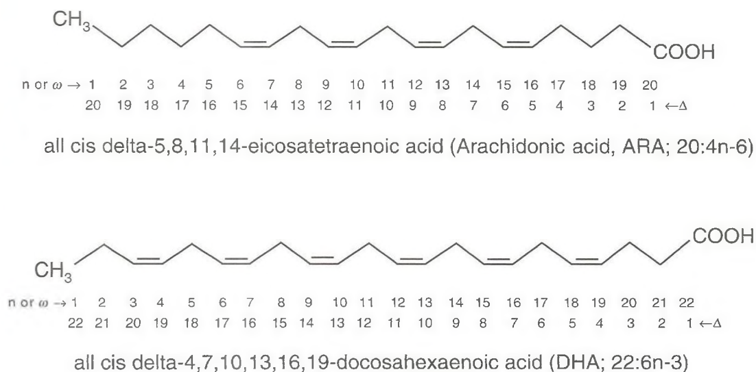
FIGURE 6-2 Arachidonic (20:4n-6) and docosahexaenoic (22:6n-3) acids showing the n and Δ carbon numbering systems.
