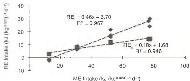
FIGURE 4-4 Recovered energy and metabolizable energy in rainbow trout, Oncorhynchus mykiss . (Recovered energy [RE] as protein [RE p , squares] and lipid [RE l , diamonds] as a function of metabolizable energy [ME] intake of rainbow trout reared at 8.5°C [data from Bureau et al., 2006]).
