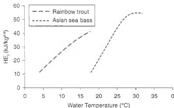
FIGURE 4-2 Fasting heat losses of rainbow trout, Oncorhynchus mykiss , and Asian sea bass, Lates calcarifer (expressed as H_E , kJ per kg^{0.8} per day and as a function of water temperature).
