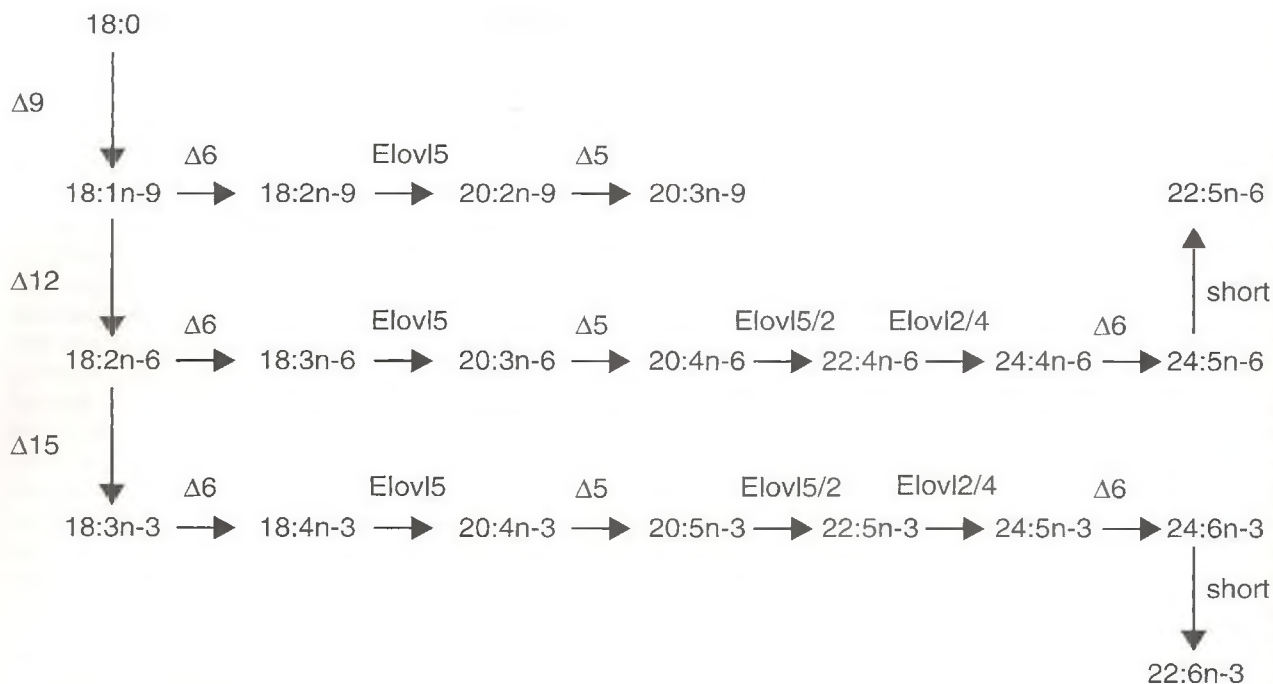
FIGURE 6-5 Pathways of biosynthesis of C20 and C22 long-chain polyunsaturated fatty acids (LC-PUFA) from n-3, n-6, and n-9 C 18 PUFA. \Delta 9 , stearoyl CoA desaturase (SCD); \Delta 5 and \Delta 6 , front-end fatty acyl desaturases (Fad). Evidence suggests that the same \Delta 6 Fad operates on both C 18 and C 24 fatty acyl substrates; \Delta 12 and \Delta 15 , Fads found only in plants and some invertebrates, and hence 18:2n-6 and 18:3n-3 cannot be formed in any vertebrate; Elov12, Elov14, and Elov15, PUFA elongases; short, peroxisomal chain shortening.
