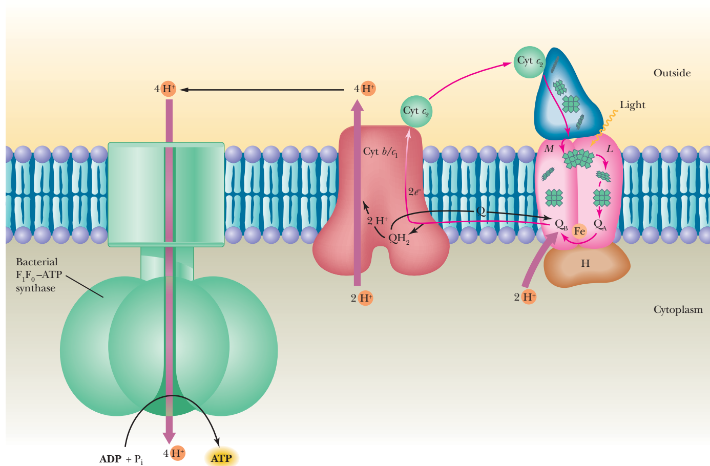
CENGAGENOW™ ACTIVE FIGURE 21.15 Photophosphorylation. Photoexcitation of the R. viridis RC leads to reduction of a quinone, Q , to form QH_2 . Oxidation of QH_2 by the cytochrome bc_1 complex leads to H^+ translocation for ATP synthesis by the R. viridis F_1F_0 -ATP synthase. Test yourself on the concepts in this figure at www.cengage.com/login .
