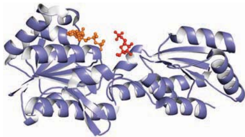
Phosphofructokinase with ADP (in orange) and fructose-6-phosphate (in red) (pdb id = 4PFK).
