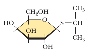
FIGURE 29.10 The structure of IPTG (isopropyl β-thiogalactoside).
