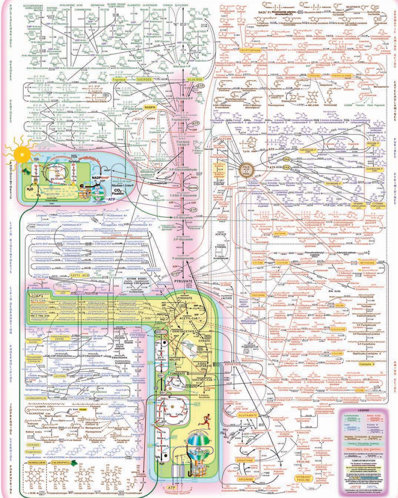
CENGAGENOW™ ANIMATED FIGURE 17.2 A metabolic map, indicating the reactions of intermediary metabolism and the enzymes that catalyze them. More than 500 different chemical intermediates, or metabolites, and a greater number of enzymes are represented here. (Source: From Donald Nicholson, Map #22, © International Union of Biochemistry and Molecular Biology.) See this figure animated at www.cengage.com/login .
