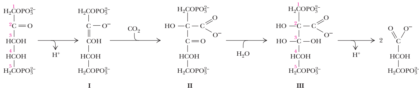
FIGURE 21.23 The ribulose biphosphate carboxylase reaction. \text{Mg}^{2+} at the active site aids in stabilizing the 2,3-enediol transition state (I) for \text{CO}_2 addition and in facilitating the carbon-carbon bond cleavage that leads to product formation.
