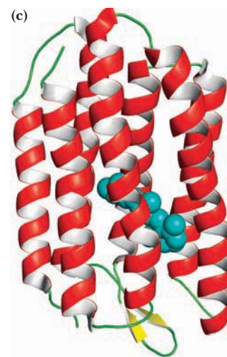
Bacteriorhodopsin, a membrane protein
