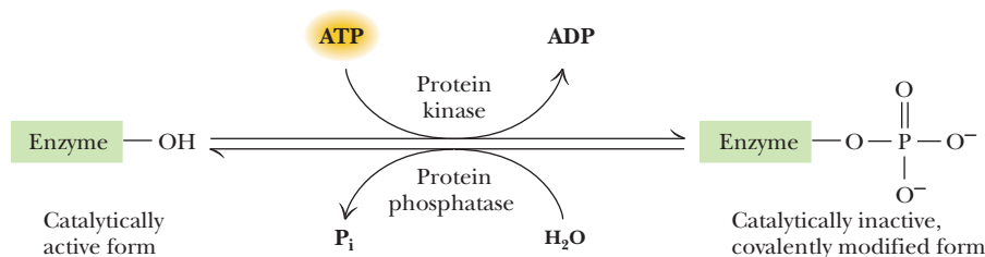
FIGURE 15.1 Enzyme regulation by reversible covalent modification.
