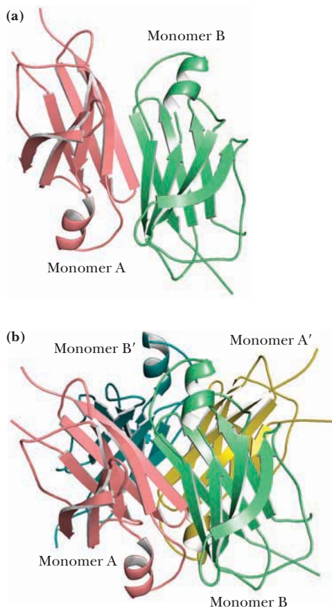
FIGURE 6.43 Many proteins form tetramers by means of two sets of isologous interactions. The dimeric (a) and tetrameric (b) forms of transthyretin (also known as prealbumin) are shown here (pdb id = 1GKE). The monomers of this protein form a dimer in a manner that extends the large monomer \beta -sheet. The tetramer is formed by isologous interactions between the large \beta -sheets of two dimers.
