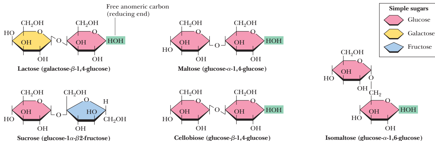
CENGAGENOW™ ACTIVE FIGURE 7.18 The structures of several important disaccharides. Note that the notation —HOH means that the configuration can be either \alpha or \beta . If the —OH group is above the ring, the configuration is termed \beta . The configuration is \alpha if the —OH group is below the ring. Also note that sucrose has no free anomeric carbon atom. Test yourself on the concepts in this figure at www.cengage.com/login .
