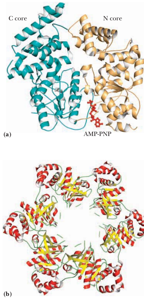
FIGURE 16.20 (a) Translocase and helicase motors of SF1 and SF2 are monomers that consist of two RecA domains in a tandem repeat (pdb id = 1QHG). (b) Motor peptides of SF3 through SF6 associate to form hexamers (as shown) or dodecamers (pdb id = 1CR0).
