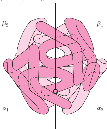
(a) Deoxyhemoglobin
