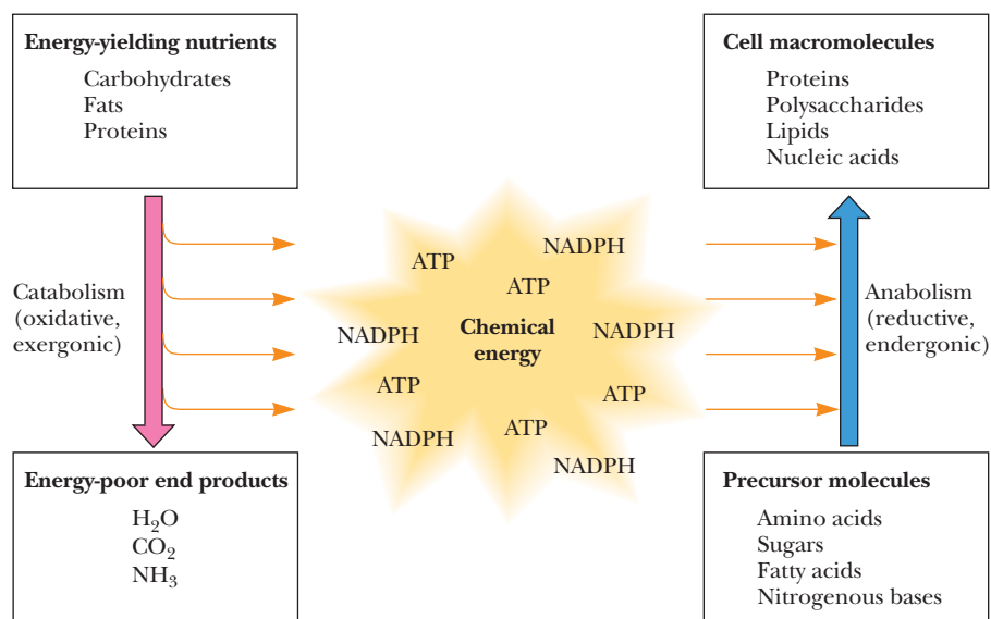
FIGURE 17.6 Energy relationships between the pathways of catabolism and anabolism. Oxidative, exergonic pathways of catabolism release free energy and reducing power that are captured in the form of ATP and NADPH, respectively. Anabolic processes are endergonic, consuming chemical energy in the form of ATP and using NADPH as a source of high-energy electrons for reductive purposes.
