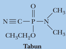
FIGURE 32.58 Covalent inhibitors of acetylcholinesterase include DIPF, the nerve gases tabun and sarin, and the insecticide malathion.
