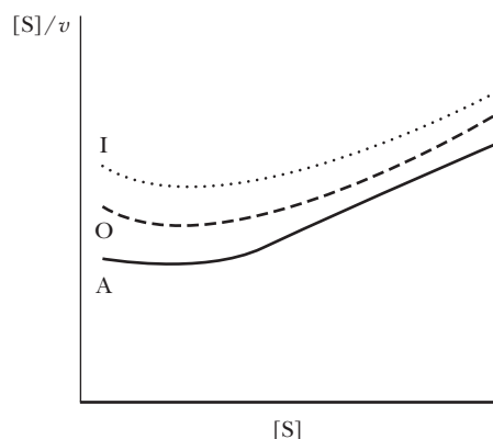
Hanes-Woolf plot
