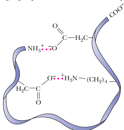
Protein strand
