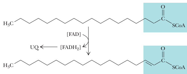
FIGURE 20.8 The fatty acyl-CoA dehydrogenase reaction, emphasizing that the reaction involves reduction of enzyme-bound FAD (indicated by brackets).
