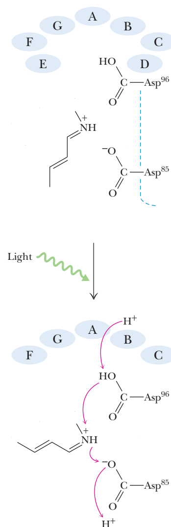
FIGURE 9.58 The mechanism of proton transport by bacteriorhodopsin. Asp 85 and Asp 96 on the third transmembrane segment (C) and the Schiff base of bound retinal serve as stepping stones for protons driven across the membrane by light-induced conformational changes. The hydrophobic environments of Asp 85 and Asp 96 raise the pK a values of their side-chain carboxyl groups, making it possible for these carboxyls to accept protons as they are transported across the membrane.
