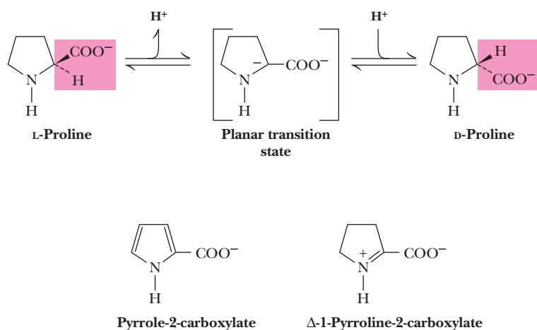
FIGURE 14.5 The proline racemase reaction. Pyrrole-2-carboxylate and \Delta -1-pyrroline-2-carboxylate mimic the planar transition state of the reaction.
