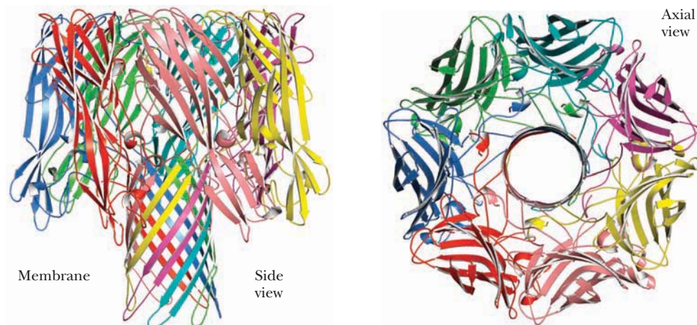
CENGAGENOW™ ACTIVE FIGURE 9.21 The structure of the heptameric channel formed by Staphylococcus aureus \alpha -hemolysin. Each of the seven subunits contributes a \beta -sheet hairpin to the transmembrane channel (pdb id = 7AHL). Test yourself on the concepts in this figure at www.cengage.com/login .
