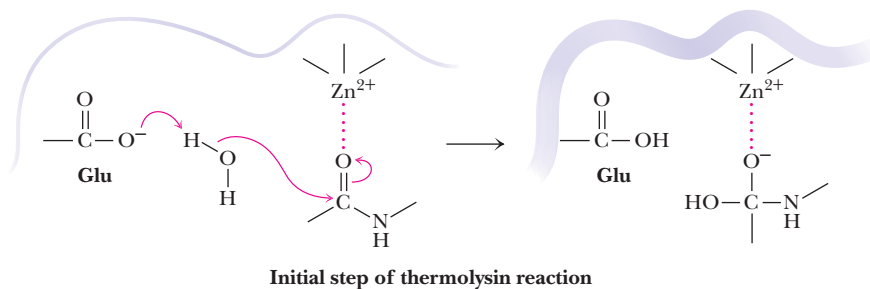
FIGURE 14.14 Thermolysin is an endoprotease (that is, it cleaves polypeptides in the middle of the chain) with a catalytic Zn^{2+} ion in the active site. The Zn^{2+} ion stabilizes the buildup of negative charge on the peptide carbonyl oxygen, as a glutamate residue deprotonates water, promoting hydroxide attack on the carbonyl carbon. Thermolysin is found in certain laundry detergents, where it is used to remove protein stains from fabrics.
