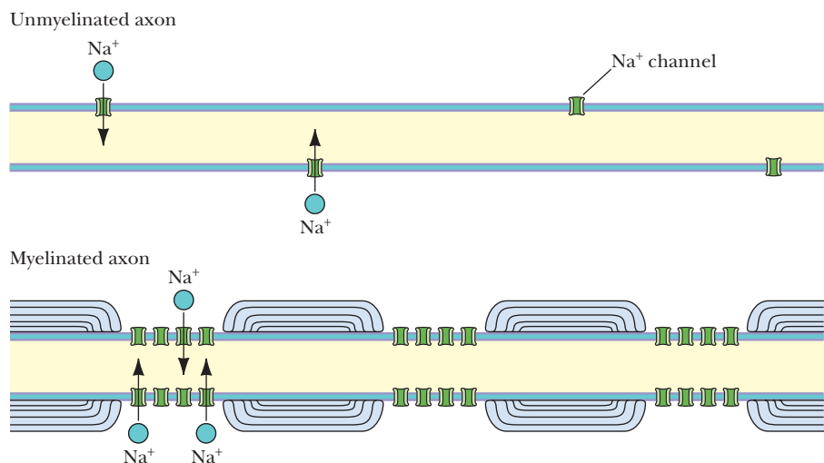
FIGURE 32.51 \text{Na}^+ channels are infrequently and randomly distributed in unmyelinated nerve. In myelinated axons, \text{Na}^+ channels are clustered in large numbers in the nodes of Ranvier, between the regions surrounded by myelin sheath structures.
