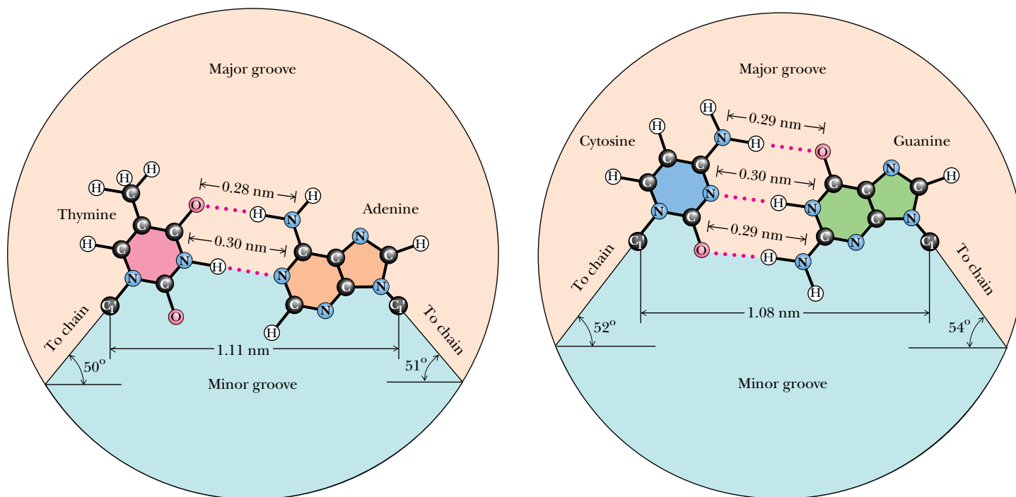
FIGURE 11.6 Watson-Crick A:T and G:C base pairs. All H bonds in both base pairs are straight.
