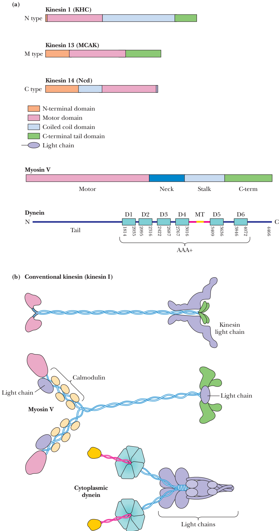
FIGURE 16.14 (a) Domain structure of kinesins, myosin V, and cytoplasmic dynein. (b) Molecular models of kinesin 1, myosin V, and cytoplasmic dynein. (Adapted from Vale, R., 2003. The molecular motor toolbox for intracellular transport. Cell 112:467–480.)
