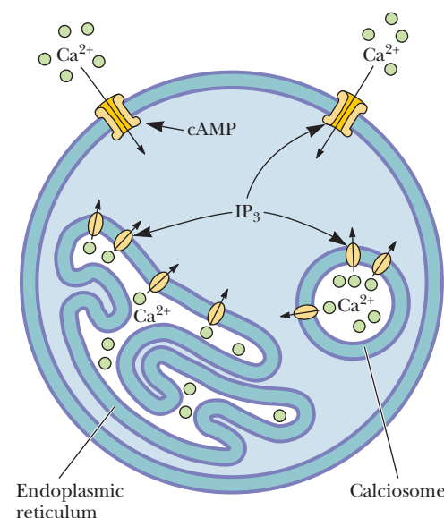
CENGAGENOW™ ANIMATED FIGURE 32.31 Cytosolic [Ca^{2+}] increases occur via the opening of Ca^{2+} channels in the membranes of calciosomes, the endoplasmic reticulum, and the plasma membrane. See this figure animated at www.cengage.com/login .
