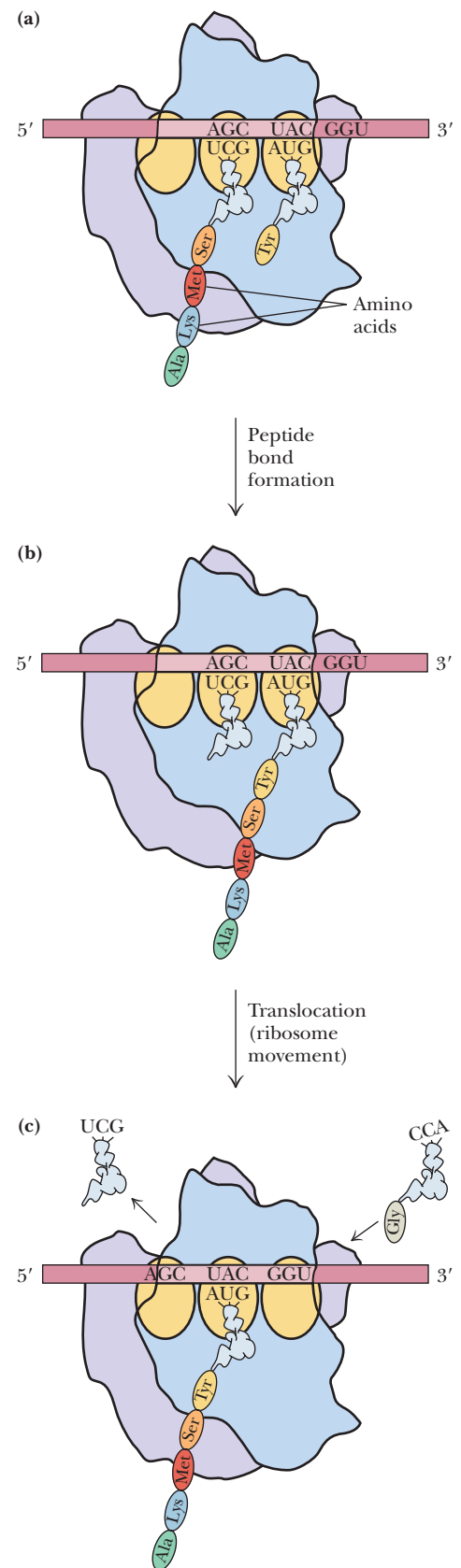
CENGAGENOW™ ACTIVE FIGURE 30.14 The basic steps in protein synthesis. The ribosome has three distinct binding sites for tRNA: the A, or acceptor, site; the P, or peptidyl, site; and the E, or exit, site. Test yourself on the concepts in this figure at www.cengage.com/login .
