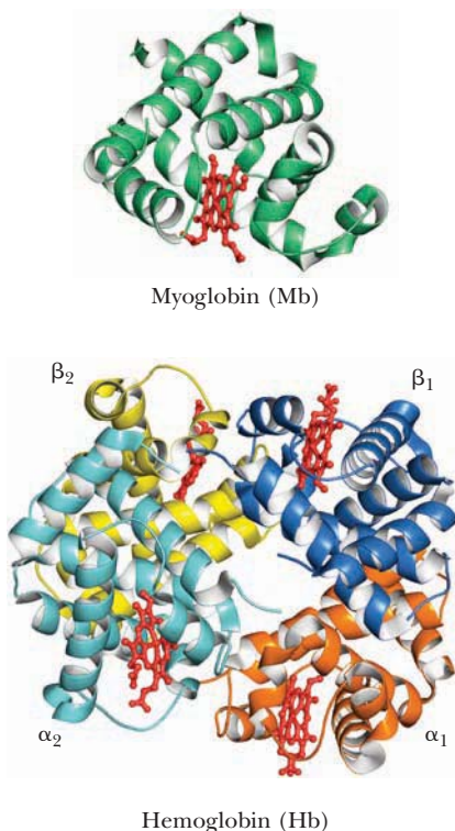
FIGURE 15.21 The myoglobin (pdb id = 2MM1) and hemoglobin (pdb id = 2HHB) molecules.
