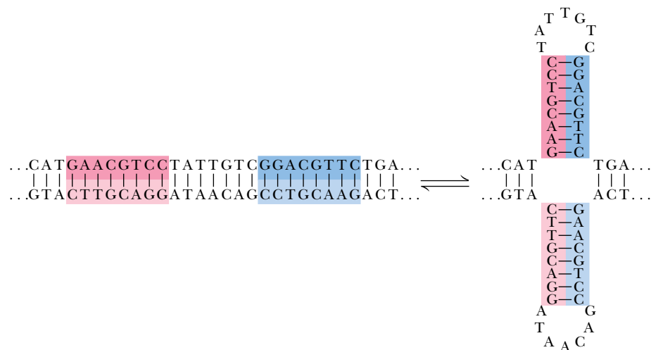
FIGURE 11.13 Self-complementary inverted repeats can rearrange to form hydrogen-bonded cruciform stem-loop structures.
