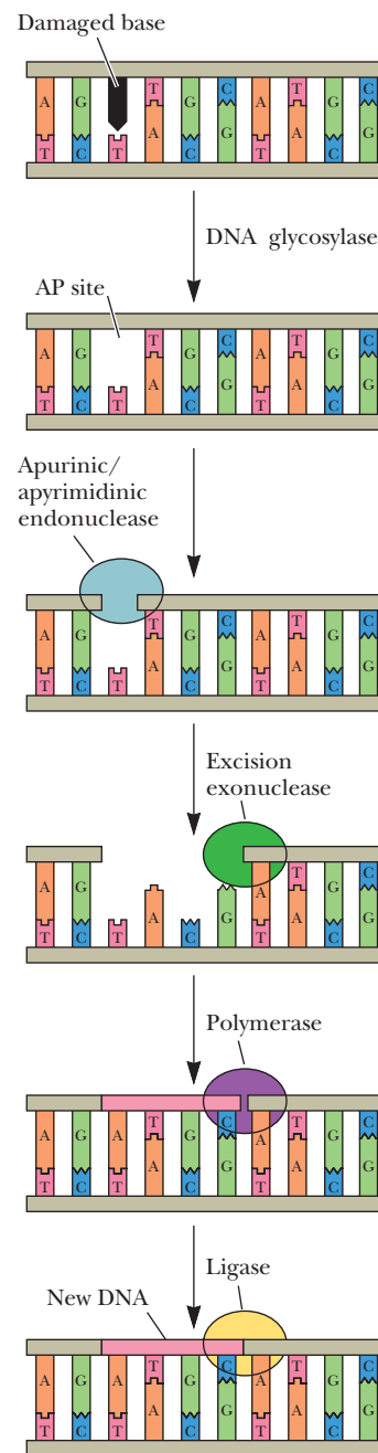
FIGURE 28.28 Base excision repair. A damaged base (■) is excised from the sugar–phosphate backbone by DNA glycosylase, creating an AP site. Then, an apurinic/apyrimidinic endonuclease severs the DNA strand, and an excision nuclease removes the AP site and several nucleotides. DNA polymerase I and DNA ligase then repair the gap.
