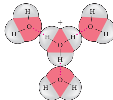
CENGAGENOW™ ANIMATED FIGURE 2.10 The hydration of \text{H}_3\text{O}^+ . See this figure animated at www.cengage.com/login
