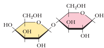
FIGURE 29.9 The structure of lactose, a β-galactoside.
