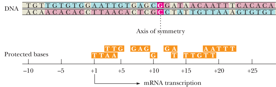
FIGURE 29.13 The nucleotide sequence of the lac operator. This sequence comprises 36 bp showing nearly palindromic symmetry. The inverted repeats that constitute this approximate twofold symmetry are shaded in rose. The bases are numbered relative to the +1 start site for transcription. The G:C base pair at position +11 represents the axis of symmetry. In vitro studies show that bound lac repressor protects a 26-bp region from –5 to +21 against nuclease digestion. Bases that interact with bound lac repressor are indicated below the operator. Note the symmetry of protection at +1 through +4 TTAA to +18 through +21 AATT.
