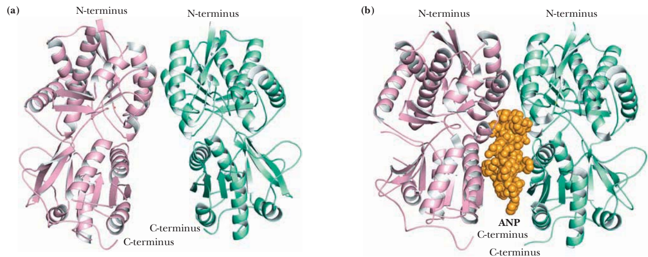
FIGURE 32.18 Activation of the ANP receptor involves binding of an asymmetric ligand at the interface of two identical receptor domains. Comparison of the structures of the receptor domain in the absence (a) and presence (b) of ANP reveals no significant intramolecular conformational change in either of the receptor monomers. ANP binding induces a twist of the two ANP receptor molecules, allowing the ANP hormone to insert between them. (a) PDB file provided by Kunio Misono, University of Nevada, Reno; (b) pdb id = 1T34.
