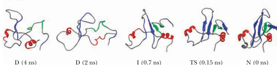
FIGURE 6.33 Computer simulations of folding and unfolding of proteins can reveal possible folding pathways. Molecular dynamics simulations of the unfolding of small proteins such as chymotrypsin inhibitor 2 (Cl2) and barnase are presented here on a reversed time scale, to show how folding may occur. D = denatured, I = intermediate, TS = transition state, N = native. (Adapted from Daggett, V., and Fersht, A. R., 2003. Is there a unifying mechanism for protein folding? Trends in Biochemical Sciences 28 :18-25. Figures provided by Alan Fersht and Valerie Daggett.)
