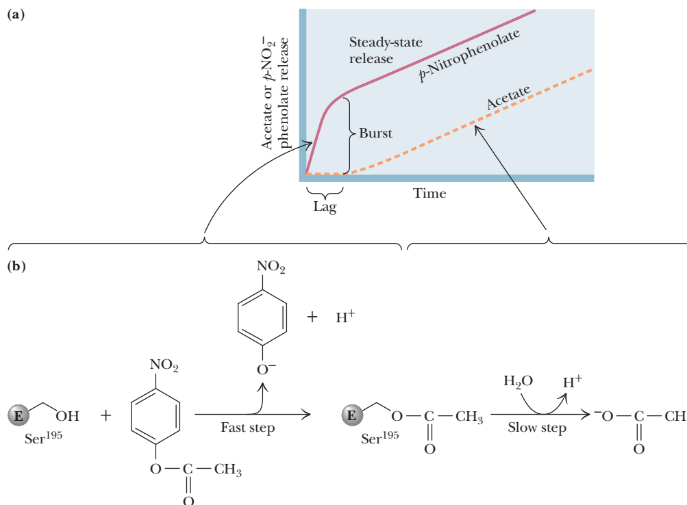
FIGURE 14.20 Burst kinetics observed in the chymotrypsin reaction (a) . A burst of nitrophenolate (b, first step) is followed by a slower, steady-state release. After an initial lag period, acetate release (b, second step) is observed. This kinetic pattern is consistent with rapid formation of an acyl-enzyme intermediate (and the burst of nitrophenolate). The slower, steady-state release of products corresponds to rate-limiting breakdown of the acyl-enzyme intermediate.
