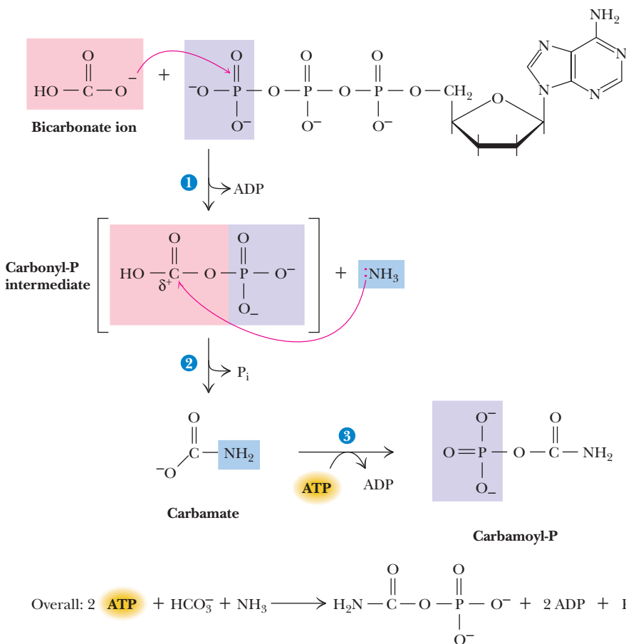
FIGURE 25.22 The mechanism of action of CPS-I.
