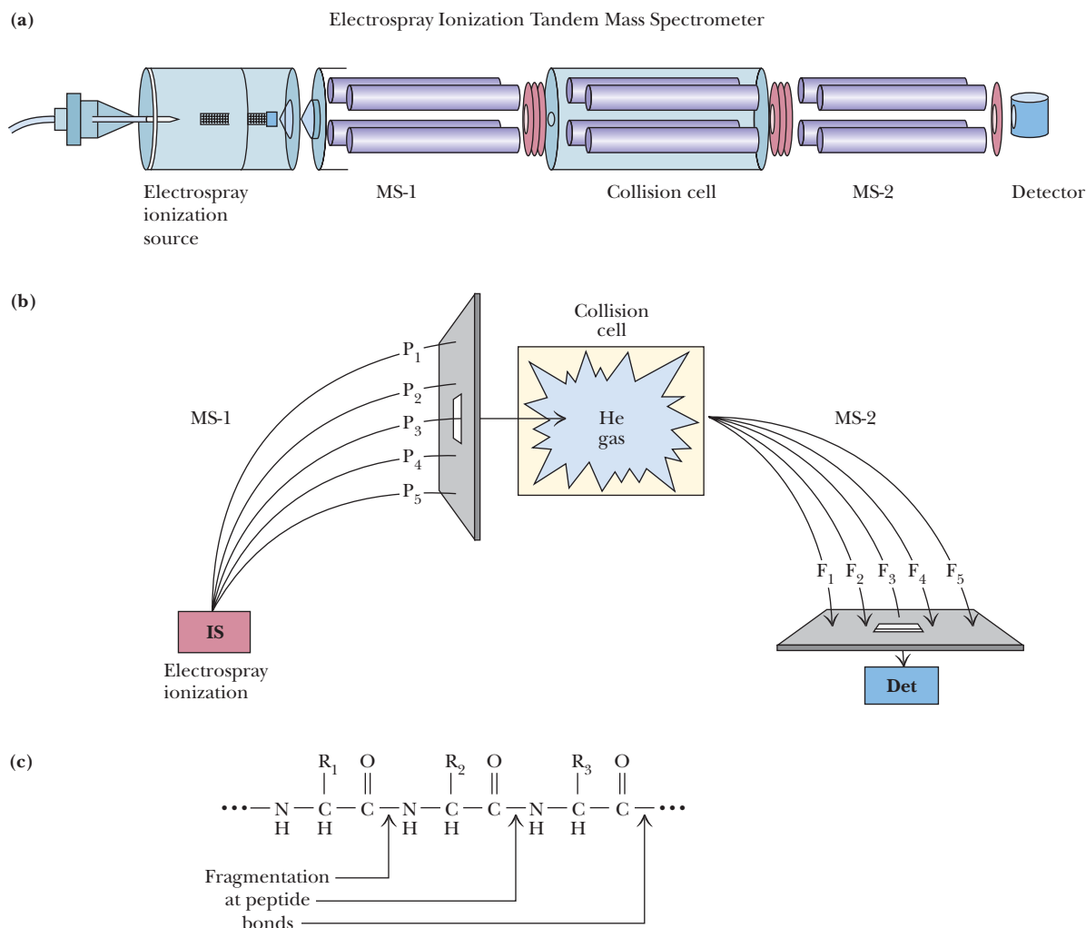
FIGURE 5.15 Tandem mass spectrometry. (a) Configuration used in tandem MS. (b) Schematic description of tandem MS: Tandem MS involves electrospray ionization of a protein digest (IS in this figure), followed by selection of a single peptide ion mass for collision with inert gas molecules (He) and mass analysis of the fragment ions resulting from the collisions. (c) Fragmentation usually occurs at peptide bonds, as indicated. (Adapted from Yates, J.R., 1996. Protein structure analysis by mass spectrometry. Methods in Enzymology 271 :351–376; and Gillece-Castro, B.L., and Stults, J.T., 1996. Peptide characterization by mass spectrometry. Methods in Enzymology 271 :427–447.)
