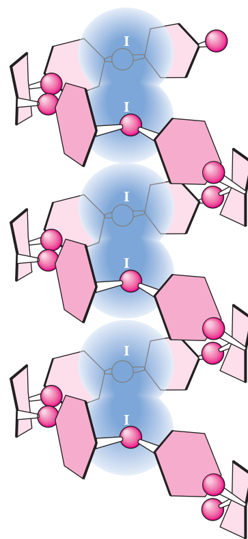
FIGURE 7.21 Suspensions of amylose in water adopt a helical conformation. Iodine ( I_2 ) can insert into the middle of the amylose helix to give a blue color that is characteristic and diagnostic for starch.
