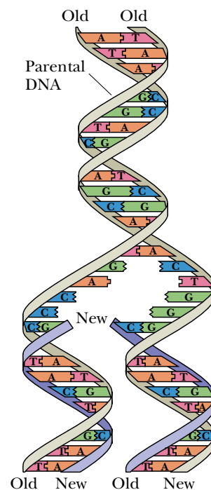
FIGURE 11.1 DNA replication yields two daughter DNA duplexes identical to the parental DNA molecule.
