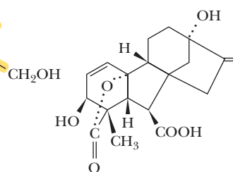
Gibberellic acid
