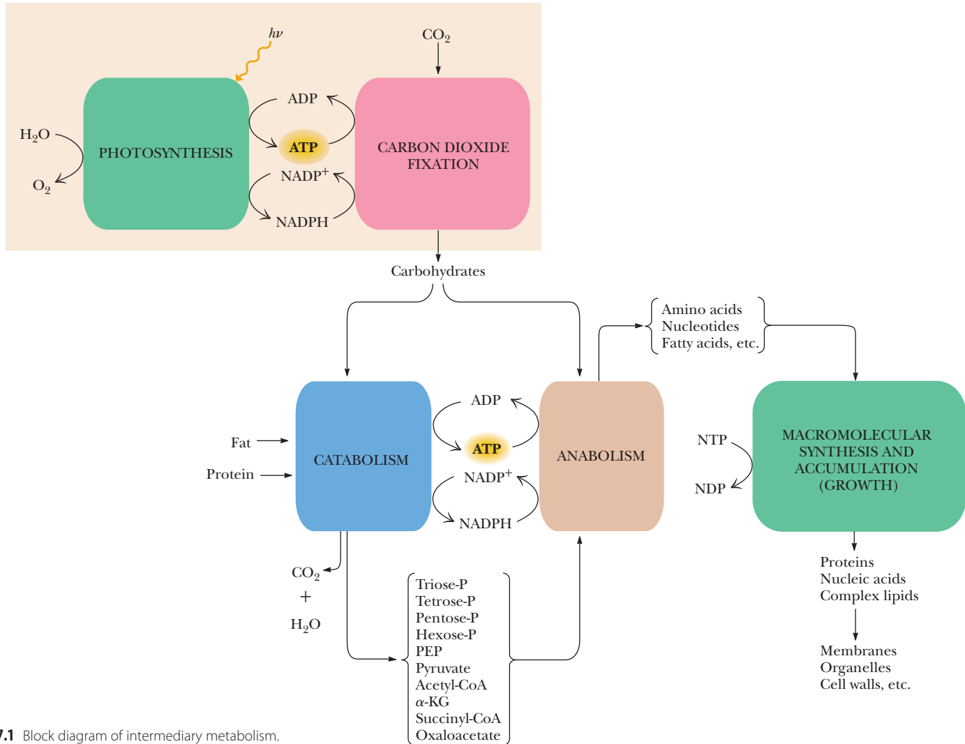
FIGURE 27.1 Block diagram of intermediary metabolism.
