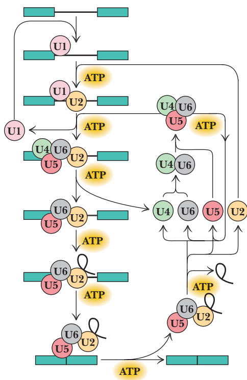
FIGURE 29.44 Events in spliceosome assembly. U1 snRNP binds at the 5'-splice site, followed by the association of U2 snRNP with the UACUAA* branch-point sequence. The triple U4/U6·U5 snRNP complex replaces U1 at the 5'-splice site and directs the juxtaposition of the branch-point sequence with the 5'-splice site, whereupon U4 snRNP is released. Lariat formation occurs, freeing the 3'-end of the 5'-exon to join with the 5'-end of the 3'-exon, followed by exon ligation. U2, U5, and U6 snRNPs dissociate from the lariat following exon ligation.
