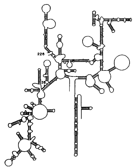
FIGURE 11.36 Comparison of secondary structures of 16S-like rRNAs from (a) a bacterium ( E. coli ), (b) an archaeon ( H. volcanii ), and (c) a eukaryote ( S. cerevisiae , a yeast).
