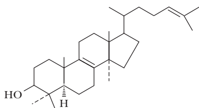
Lanosterol
