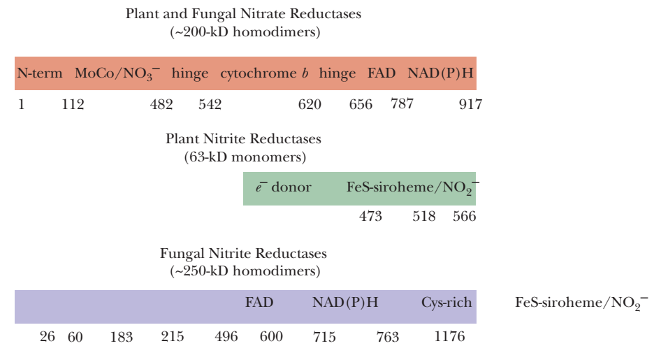
FIGURE 25.3 Domain organization within the enzymes of nitrate assimilation. The numbers denote residue number along the amino acid sequence of the proteins.
