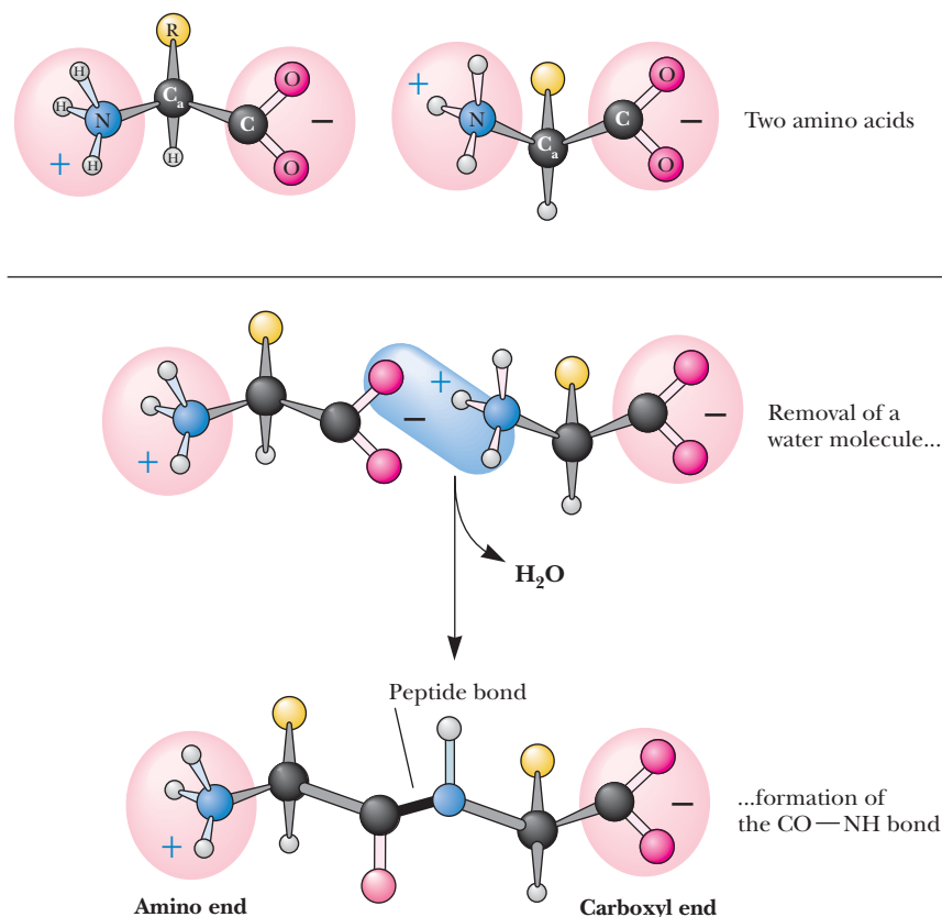
CENGAGENOW™ ANIMATED FIGURE 4.2 The \alpha\text{-COOH} and \alpha\text{-NH}_3^+ groups of two amino acids can react with the resulting loss of a water molecule to form a covalent amide bond. (Illustration: Irving Geis. Rights owned by Howard Hughes Medical Institute. Not to be reproduced without permission.) See this figure animated at www.cengage.com/login
