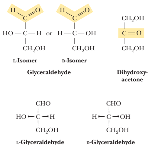
FIGURE 7.1 Structure of a simple aldose (glyceraldehyde) and a simple ketose (dihydroxyacetone).
