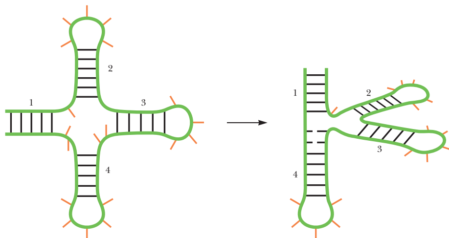
FIGURE 11.31 Junctions and coaxial stacking in RNA. Stem junctions (or multibranched loops) are another type of RNA secondary structure. Coaxial stacking of stems or stem-loops (as in stacking of stem 1 on stem-loop 4) is a tertiary structural feature found in many RNAs. (Adapted from Figure 1 in Tyagi, R., and Matthews, D. H., 2007. Predicting coaxial stacking in multibranch loops. RNA 13:1–13.)
