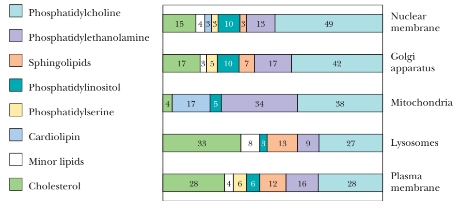
FIGURE 9.2 The lipid composition of rat liver cell membranes, in weight percent. (Adapted from Andreoli, T. E., 1987. Membrane Physiology , 2nd ed. Chapter 27, Table II, and Daum, G., 1985. Lipids of mitochondria. Biochimica et Biophysica Acta 822:1–42.)
