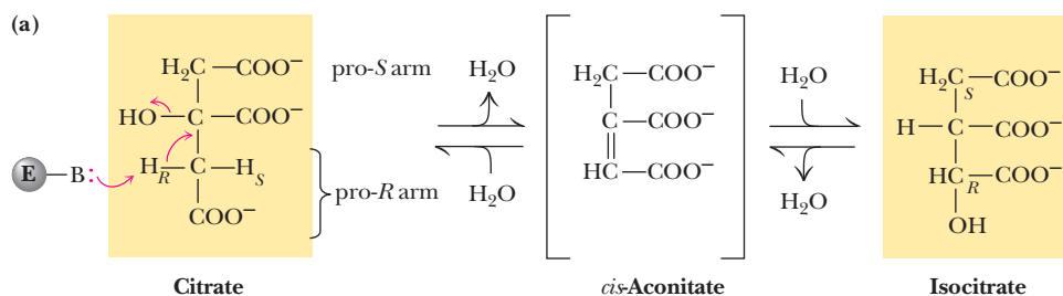
FIGURE 19.8 (a) The aconitase reaction converts citrate to cis -aconitate and then to isocitrate. Aconitase is stereospecific and removes the pro- R hydrogen from the pro- R arm of citrate. (b) The active site of aconitase. The iron–sulfur cluster (pink) is coordinated by cysteines (orange) and isocitrate (purple) (pdb id = 1B0J).
