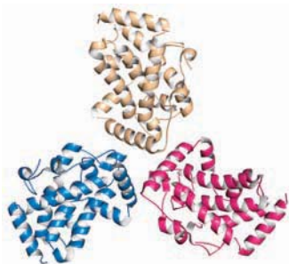
Trimer E. blattae acid phosphatase (pdb id = 2EOI)
