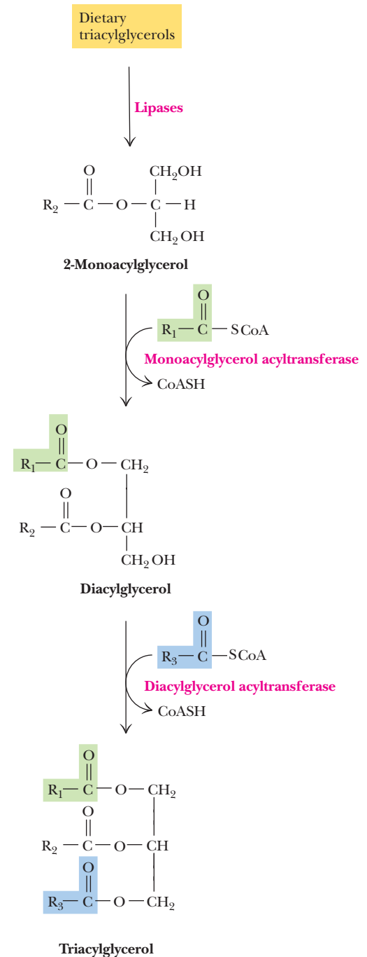
FIGURE 24.20 Triacylglycerols are formed primarily by the action of acyltransferases on monoacylglycerol and diacylglycerol.
