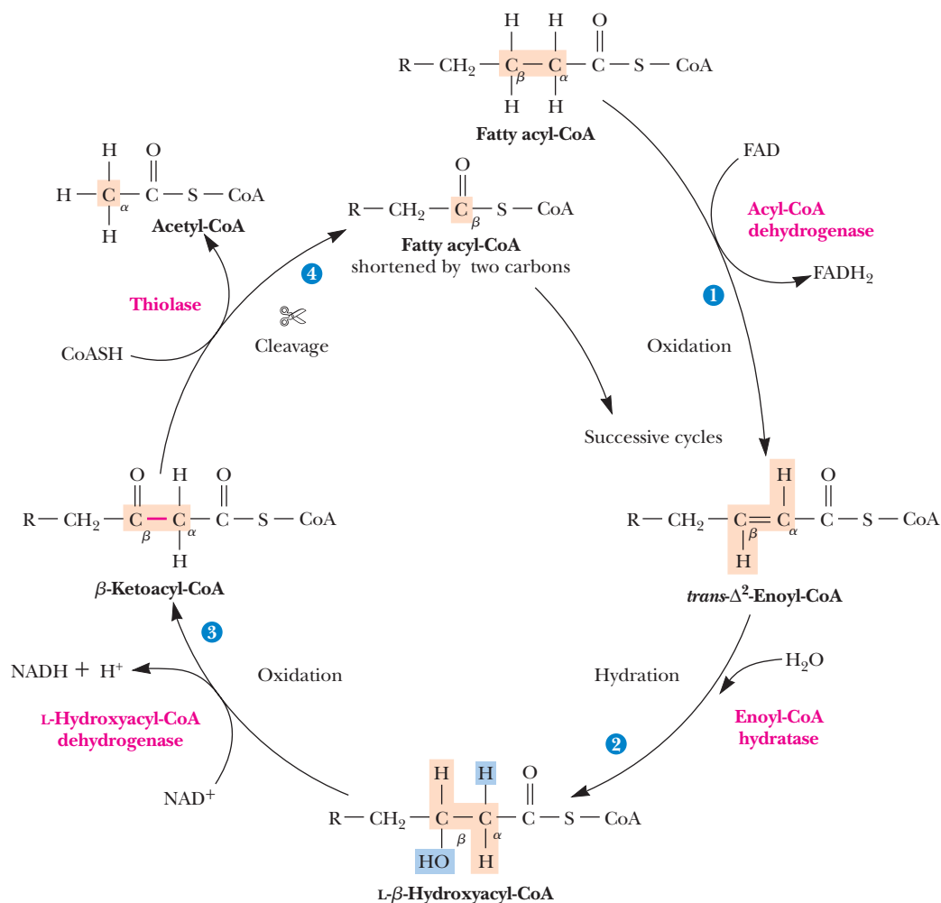
FIGURE 23.9 The \beta -oxidation of saturated fatty acids involves a cycle of four enzyme-catalyzed reactions. Each cycle produces single molecules of \text{FADH}_2 , \text{NADH} , and acetyl-CoA, consumes a water, and yields a fatty acid shortened by two carbons. (The delta [ \Delta ] symbol connotes a double bond, and its superscript indicates the lower-numbered carbon involved.)
