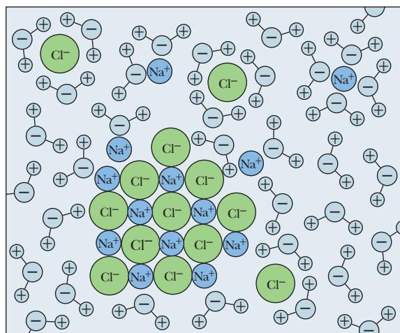
CENGAGENOW™ ANIMATED FIGURE 2.4 Hydration shells surrounding ions in solution. Water molecules orient so that the electrical charge on the ion is sequestered by the water dipole. See this figure animated at www.cengage.com/login
