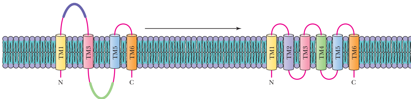
(a) Aquaporin-1
