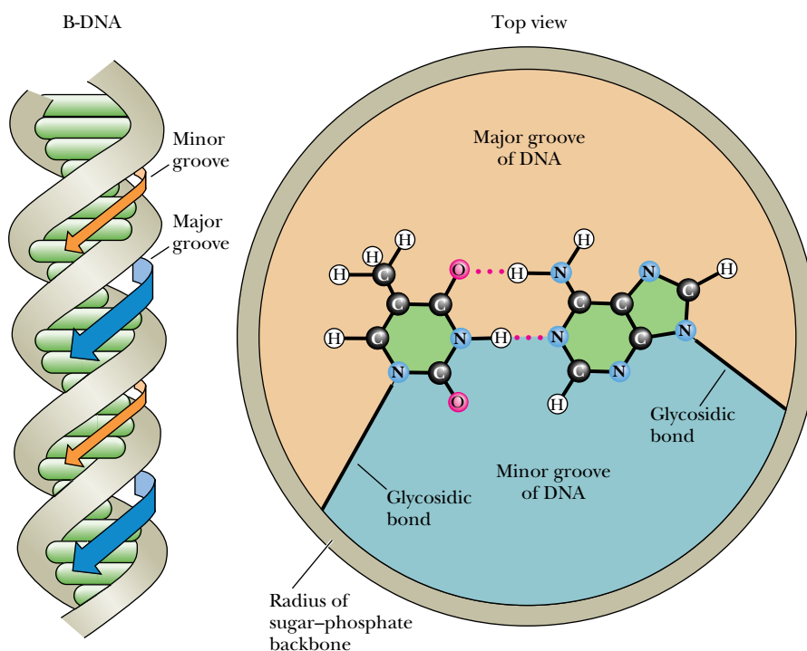
FIGURE 11.7 The major and minor grooves of B-DNA.
