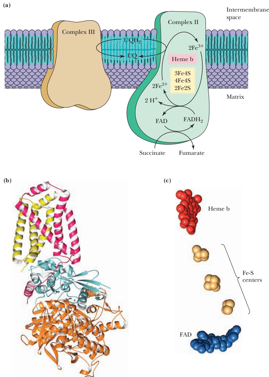
CENGAGENOW™ ACTIVE FIGURE 20.7 (a) A scheme for electron flow in Complex II. Oxidation of succinate occurs with reduction of [FAD]. Electrons are then passed to Fe-S centers and then to coenzyme Q (UQ). Proton transport does not occur in this complex. (b) The structure of Complex II from pig heart (pdb id = 1ZOY). (c) The arrangement of redox centers. Electron flow is from bottom to top. Test yourself on the concepts in this figure at www.cengage.com/login .
