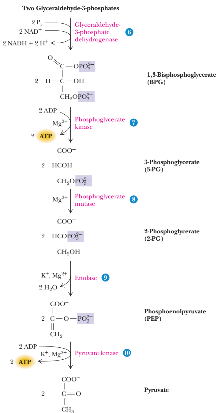
CENGAGENOW™ ACTIVE FIGURE 18.1 The glycolytic pathway. Test yourself on the concepts in this figure at www.cengage.com/login .
