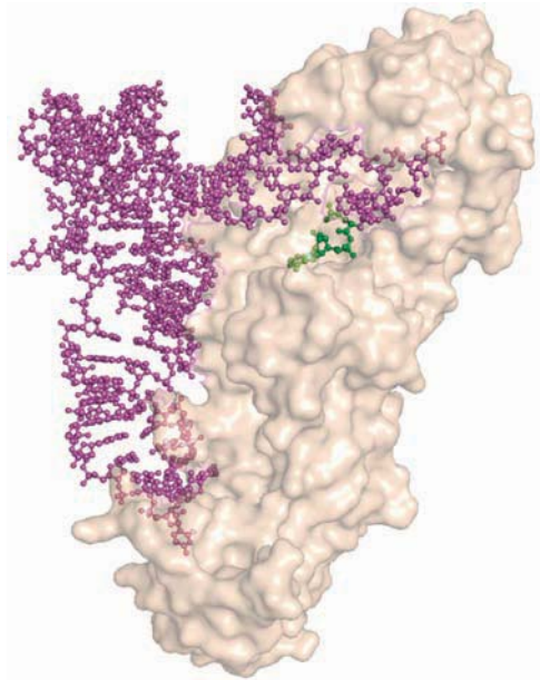
FIGURE 30.7 Structure of E. coli glutamyl-tRNA Gln synthetase complexed with tRNA Gln and ATP (pdb id = 1GSG). The protein: tRNA contact region extends along one side of the entire length of this extended protein. The acceptor stem of the tRNA and the ATP (green) fit into a cleft at the top of the protein in this view. The enzyme also interacts extensively with the anticodon (lower tip of tRNA Gln ).
