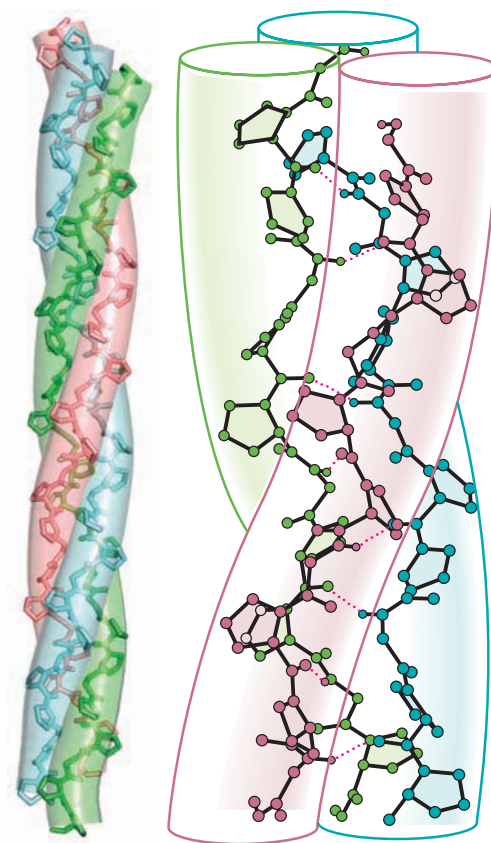
CENGAGENOW™ ACTIVE FIGURE 6.16 Poly(Gly-Pro-Pro), a collagenlike right-handed triple helix composed of three left-handed helical chains (pdb id = 1K6F). (Adapted from Miller, M. H., and Scheraga, H. A., 1976. Calculation of the structures of collagen models. Role of interchain interactions in determining the triple-helical coiled-coil conformation. I. Poly(glycyl-prolyl-prolyl). Journal of Polymer Science Symposium 54:171–200.) Test yourself on the concepts in this figure at www.cengage.com/login .
