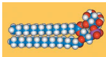
CENGAGENOW™ ANIMATED FIGURE 8.6 Structures of several glycerophospholipids and space-filling models of phosphatidylcholine, phosphatidylglycerol, and phosphatidylinositol. See this figure animated at www.cengage.com/login .
