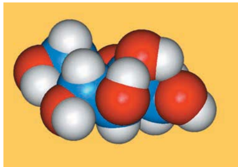
\beta -D-Fructofuranose
