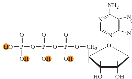
FIGURE 3.13 Adenosine-5'-triphosphate (ATP).
