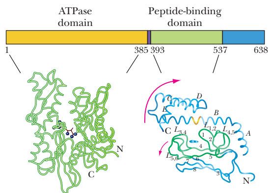
FIGURE 31.2 Structure and function of DnaK: (a) Domain organization and structure of the Hsp70 family member, DnaK. The ribbon diagram on the lower left is the ATP-binding domain of the DnaK analog, bovine Hsc70; bound ADP is shown as a stick diagram (purple). The ribbon diagram on the lower right is the polypeptide-binding domain of DnaK. The small blue ovals highlight the position of the polypeptide substrate; the protein regions that bind the polypeptide substrate are blue-green. (b) DnaK mechanism of action: DnaJ binds an unfolded protein (U) or partially folded intermediate (I) and delivers it to the DnaK:ATP complex. The nucleotide exchange protein GrpE replaces ADP with ATP on DnaK and the partially folded intermediate (II) is released. I has several possible fates: It may fold into the native state, N; it may undergo another cycle of interaction with DnaJ and DnaK; or it may become a substrate for folding by the GroEL chaperonin system. (Adapted from Figures 1a and 2a in Frydman, J., 2001. Folding of newly translated proteins in vivo: The role of molecular chaperones. Annual Review of Biochemistry 70 :603–647.)
