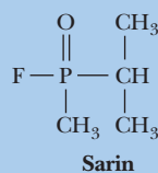
FIGURE 32.58 Covalent inhibitors of acetylcholinesterase include DIPF, the nerve gases tabun and sarin, and the insecticide malathion.
