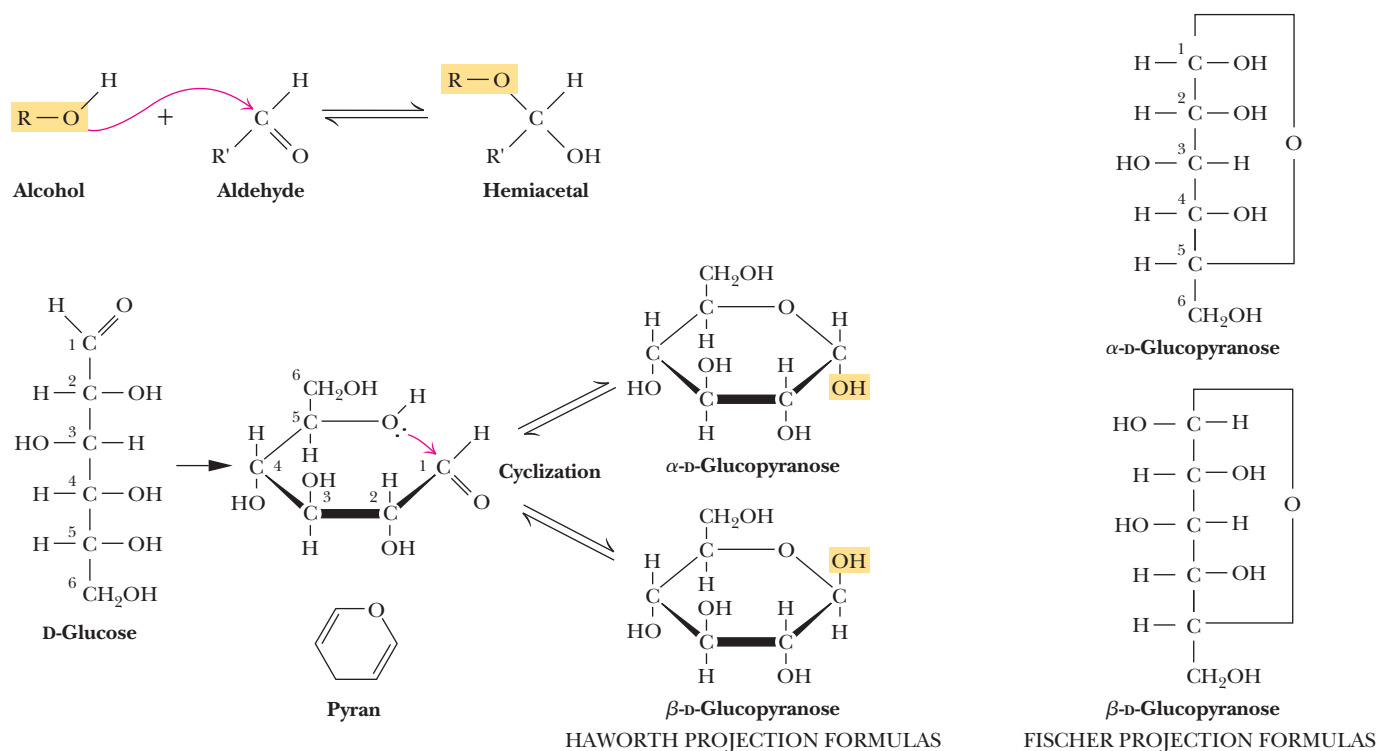
CENGAGENOW™ ANIMATED FIGURE 7.5 The linear form of D-glucose undergoes an intramolecular reaction to form a cyclic hemiacetal. See this figure animated at www.cengage.com/login .
