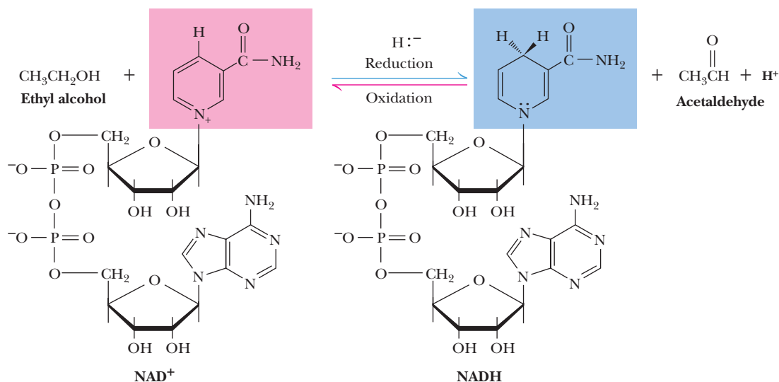
FIGURE 17.11 Hydrogen and electrons released in the course of oxidative catabolism are transferred as hydride ions to the pyridine nucleotide, \text{NAD}^+ , to form \text{NADH} + \text{H}^+ in dehydrogenase reactions of the type
