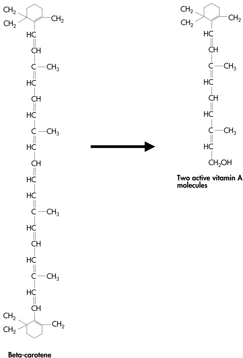
Figure 5-1 Conversion of beta-carotene to vitamin A.
