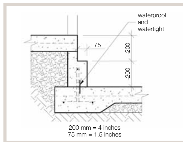
Figure A4.6 Foundation designed to be watertight (dimensions metric).
